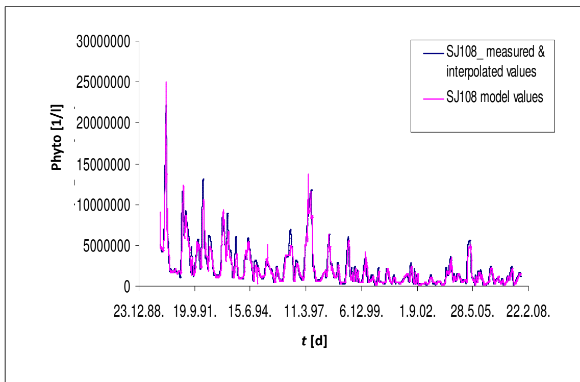
Figure 5.11 Results of (3 rd ) model for station SJ108 vs. measured & interpolated values (R= 0.72)
