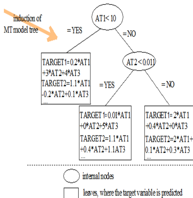
Figure 3.3 Induction of multi target model trees from given data set (examples)
