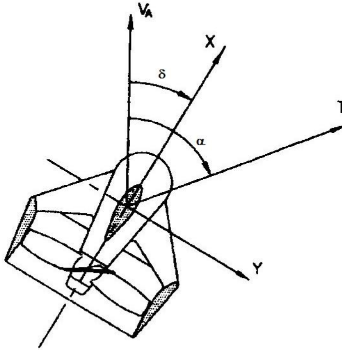
Figure 4.8: Reference system for a thruster in cross-flow [25]
