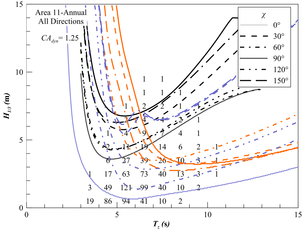
Figure 6.13: Critical curves according to different criteria: DP ( black ), pitch ( orange ) and roll ( purple ) on a generic PLV vessel.
