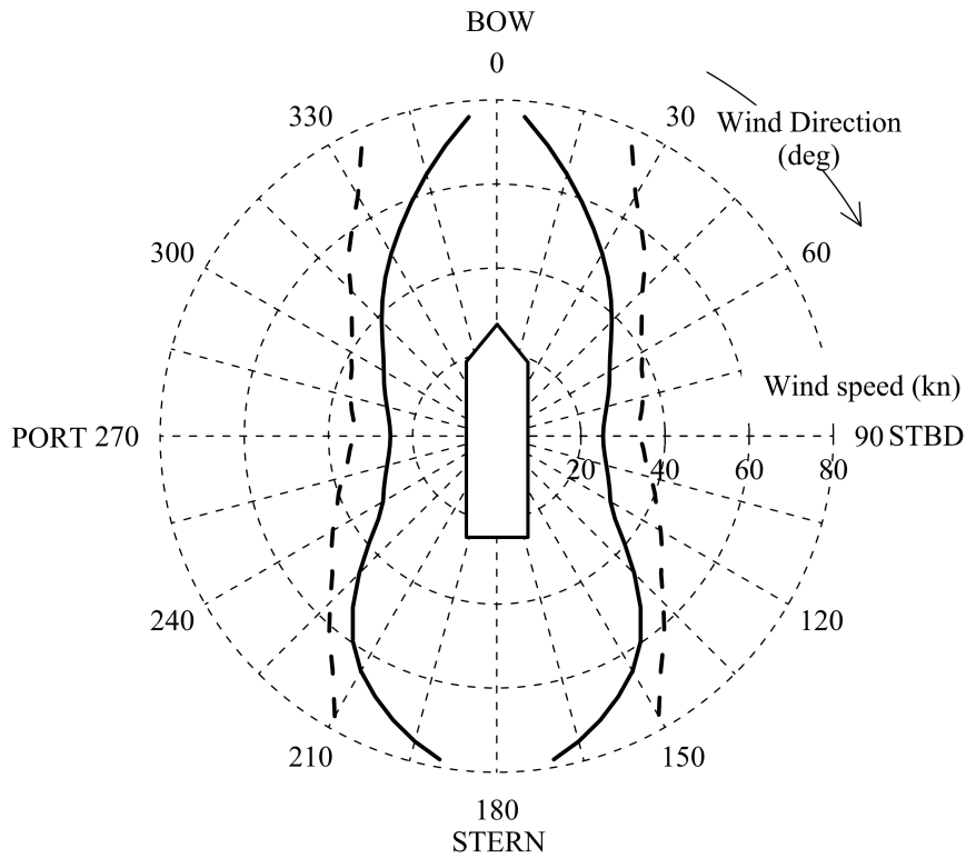
Figure 2.7: Comparison between quasi-steady ( dotted ) and time domain ( continuous ) simulations for the Drill-ship test case, considering Pierson-Moskowitz wind-wave correlation
