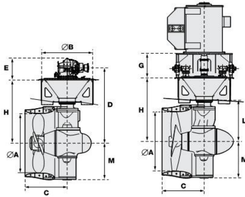
Figure 4.1: Example of steerable thruster in Z-drive (left) and L-drive (right) configuration [149]
