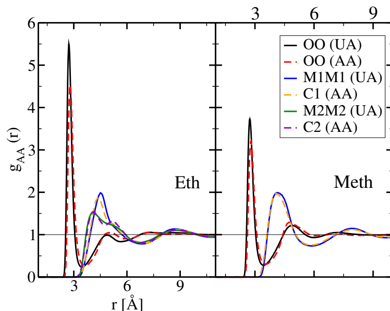
Figure A.4.: Selected site-site RDFs for pure ethanol (left panel) and pure methanol (right panel). The united atom (full lines) and all atom (dashed lines) are compared.
