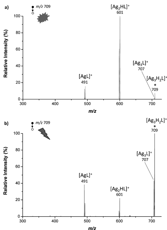
Figure 2. MS^2 spectra showing the fragmentation of the [Ag_3H_2L]^+ ion ( m/z 709) under conditions of: a) CID with a NCE of 25%, b) laser-induced dissociation (LID) at 260 nm with five laser shots; *: the mass selected precursor ions. A window of 1.3 Th was used to isolate a single peak from the isotope cluster, corresponding to [^{107}Ag_2^{109}AgH_2L]^+ .
