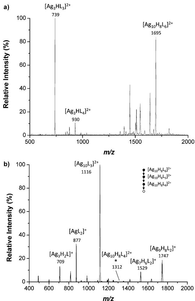
Figure 1. a) Full ESI/MS of silver hydride nanocluster ions synthesised from reaction of AgNO_3 with NaBH_4 . b) MS^2 CID spectrum of [Ag_{10}H_8L_4]^{2+} ion ( m/z 1312), which was mass selected with a window of 20 Th to allow isolation of the full distribution of ^{107}Ag and ^{109}Ag isotopes. A NCE of 10% was used to dissociate the cluster and the m/z values of the products ions indicate the most intense peak in the cluster as a result of the various combination of the silver(I) isotopes; *: the mass selected precursor ion.
