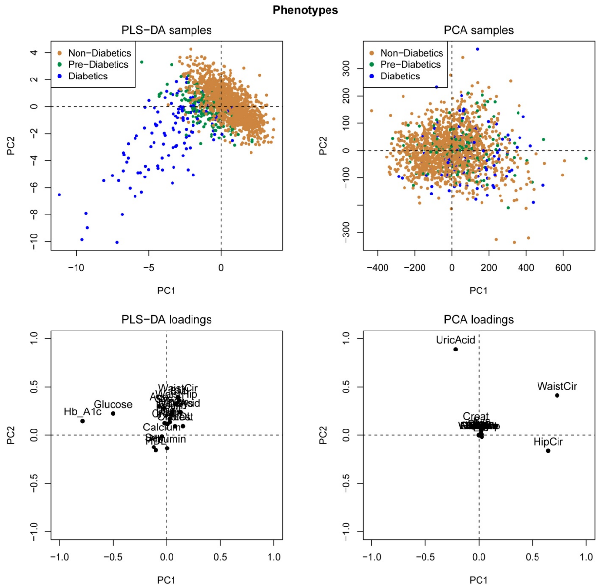
Figure 19. PLS-DA and PCA analysis of the diabetes groups using phenotype data. Although PLS-DA achieved a separation of the groups and HbA1c and glucose were indicated as the most important factors for the separation, PCA was not able to distinguish the groups. The score plots representing the data samples by the two first principal components (PC1 on the x-axis and PC2 on the y-axis) are shown on the upper panels; groups are coloured as gold for non-diabetic, green for pre-diabetic and blue for diabetic. The corresponding loading plots establishing the relative contributions of each phenotype feature to the overall variation in the groups are shown on the lower panels.
