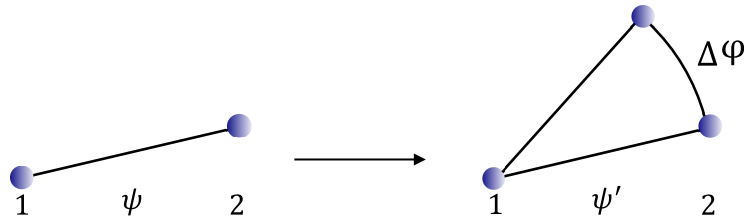
Figure 1.1: Particle 2 moves around particle 1 by an angle \Delta\phi .
