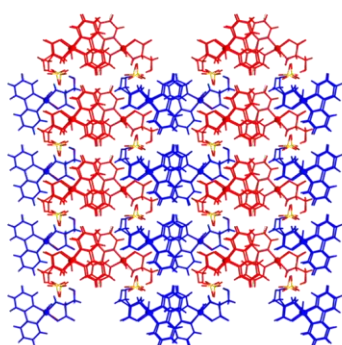
\beta -11a
