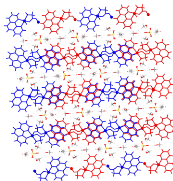
10b·6CH 3 OH
