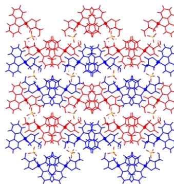
\alpha -11a
