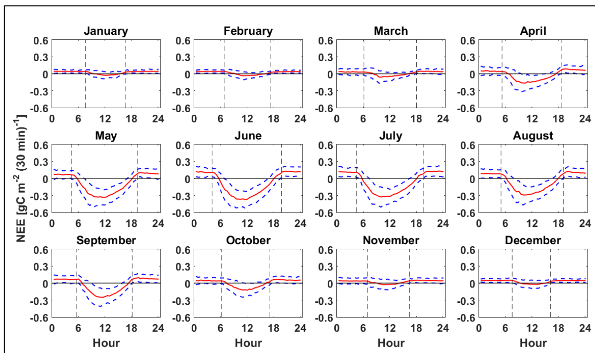
Figure 4.11: Mean diurnal variation of NEE by months during the years 2008 to 2017; blue dashed line marks 1 standard deviation; vertical dashed line marks the time of sunrise and sunset on the 15 th day of the month
