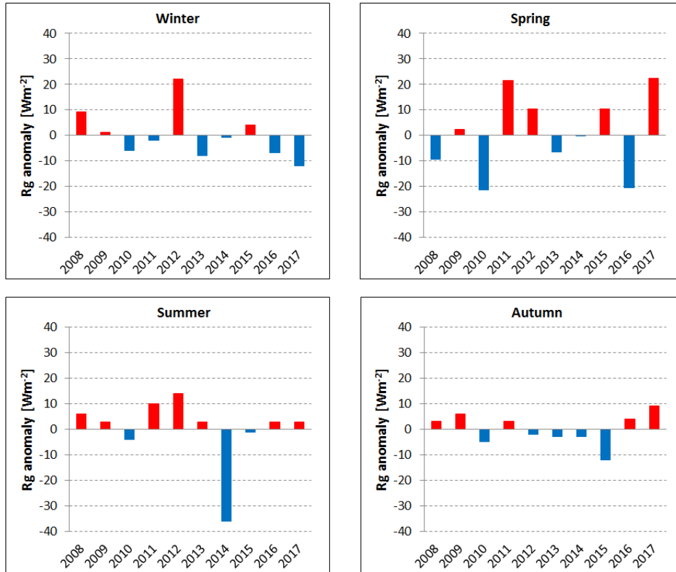
Figure 4.23: Seasonal anomalies of R_g [ \text{W m}^{-2} ], 2008-2017
