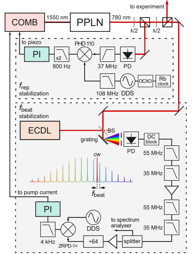
FIG. 1. Sketch of the experimental setup for fully stabilizing the comb using an ECDL. The upper and lower section of the image shows the scheme for stabilizing f_{rep} and f_{beat} , respectively. The DDS's in the upper and lower part of the figure are the same unit. The spectrum after the grating is an illustration, in reality it does not stretch to the visible part of the spectrum. The setup does not require an iris, the spatial filtering is achieved due to the photodiode active area being small. PPLN: periodically poled lithium niobate crystal, PD - photodiode, \lambda/2 - half-wave plate, DDS - direct digital synthesizer, OCXO - oven controlled crystal oscillator, ECDL - external cavity diode laser, BS - beam splitter.
