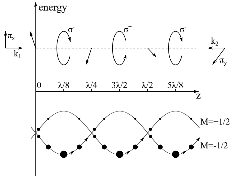
Figure 2.3: Polarization gradient cooling in the \text{lin} \perp \text{lin} case. The spatial dependence of the light shift is shown as is the polarization of the corresponding field, upper part of the image. The size of the black circles represents the population fraction in the two substates. We can see that the majority of the population will be in the substate with the lower energy due to optical pumping and that this population will have an upward climb toward the "node" of the potential where the populations are the same in the two sublevels. Adapted from [1, 47]
