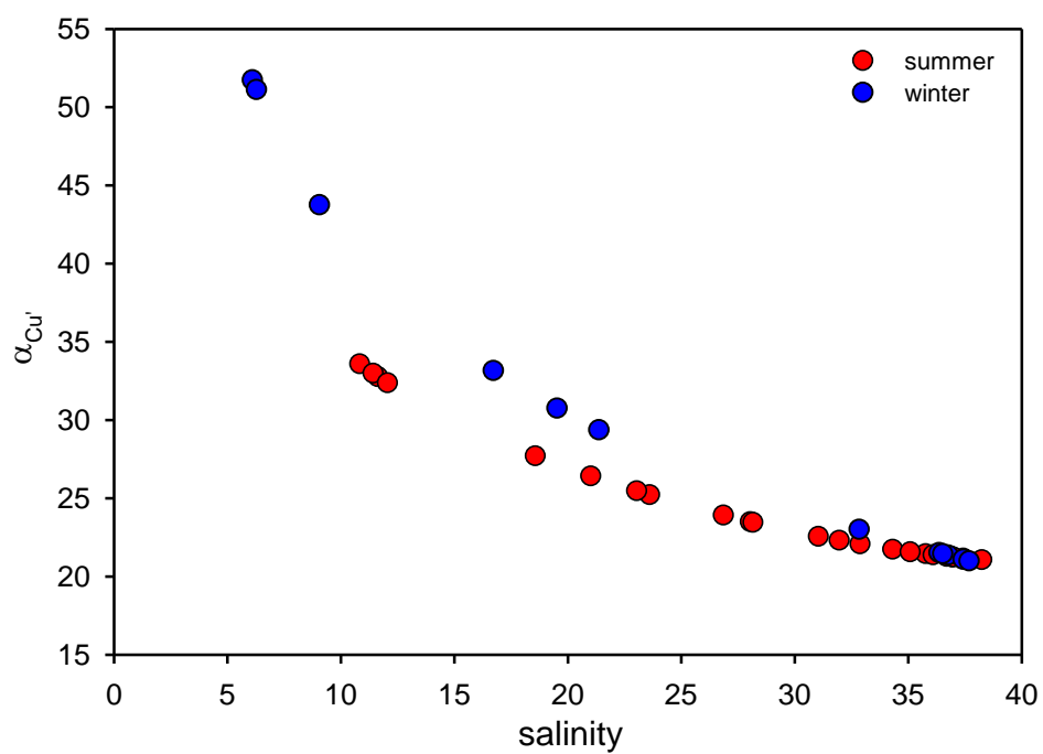
Figure 4.37. Dependence of the inorganic side reaction coefficients of Cu ( \alpha_{Cu'} ) on salinity calculated for summer (red) and winter (blue) samples.
