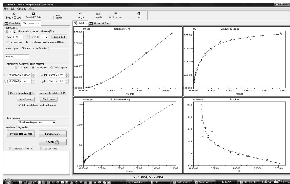
Figure 2.18. Snapshot of ProMCC software showing plots of titration curve (top left), Langmuir/Geringa (top right), R/VDB (bottom left) and Scatchard (bottom right) plots. Data were fitted applying R/VDB log-log fitting routine (blue curve).
