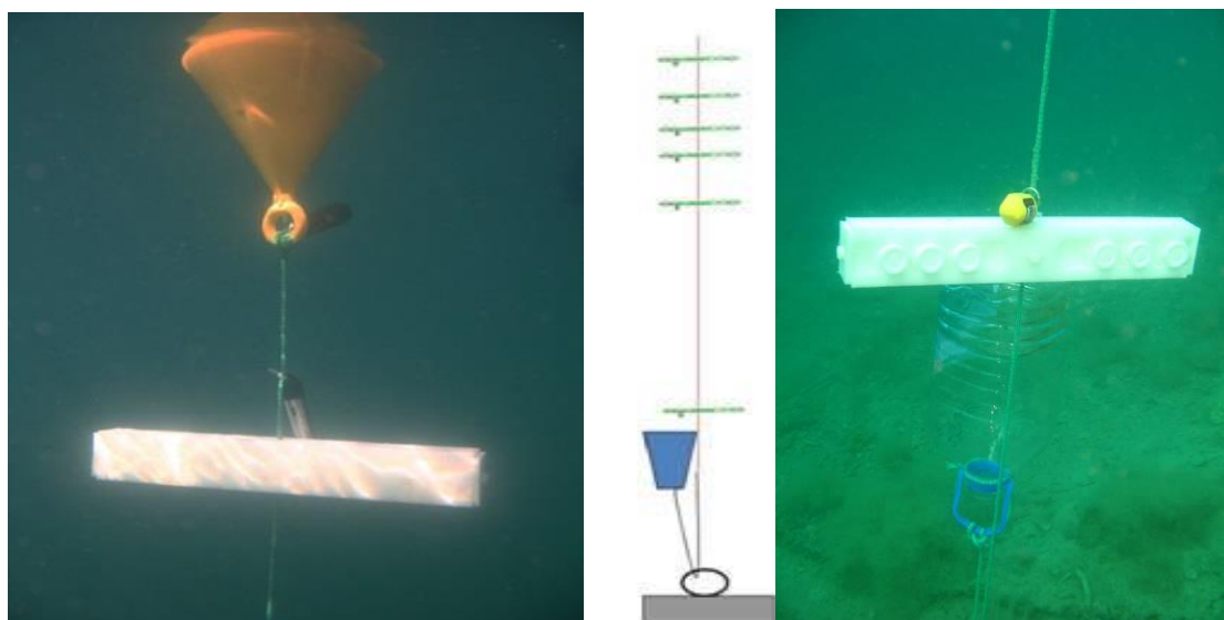
Figure 3.9. Buoy at the surface to which the rope was attached (left) and shematic representation and actual photo of the counter-weight (right) with holder filled with 3-replicates of OP-DGT and RP-DGT (at 8 m)
