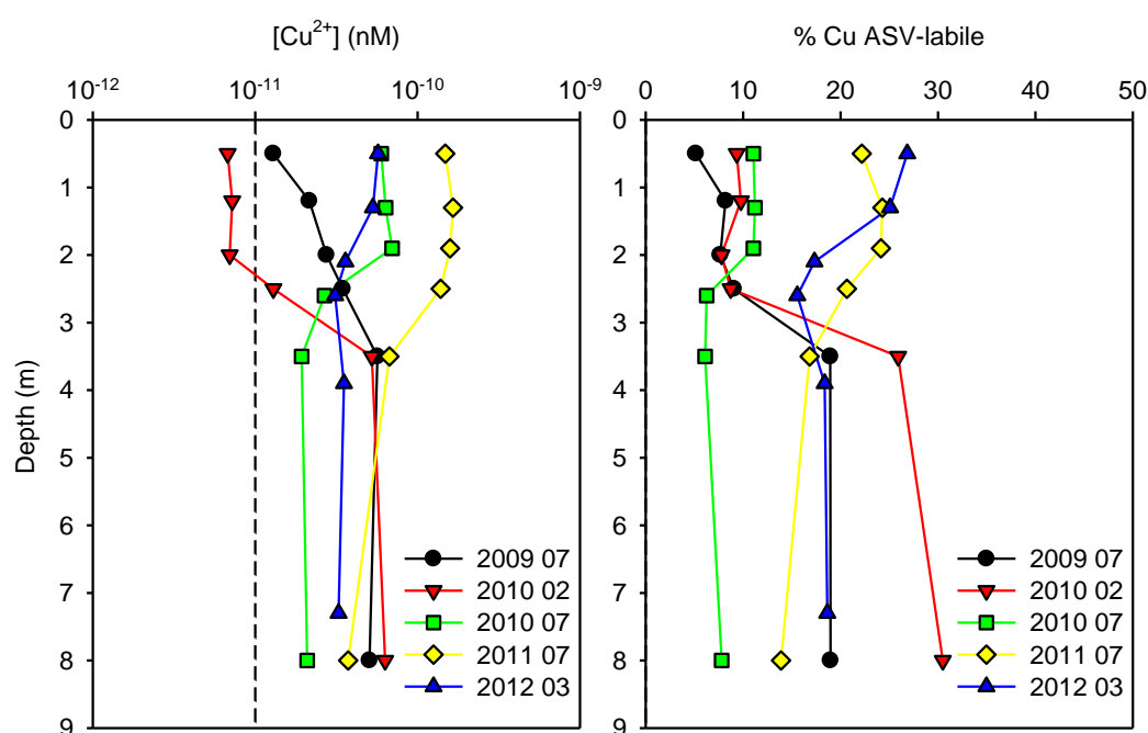
Figure 5.21. Vertical distribution of calculated free Cu concentration ( [\text{Cu}^{2+}] ) (left plot) and percentage of ASV-labile copper (right plot) for all sampling campaigns.
