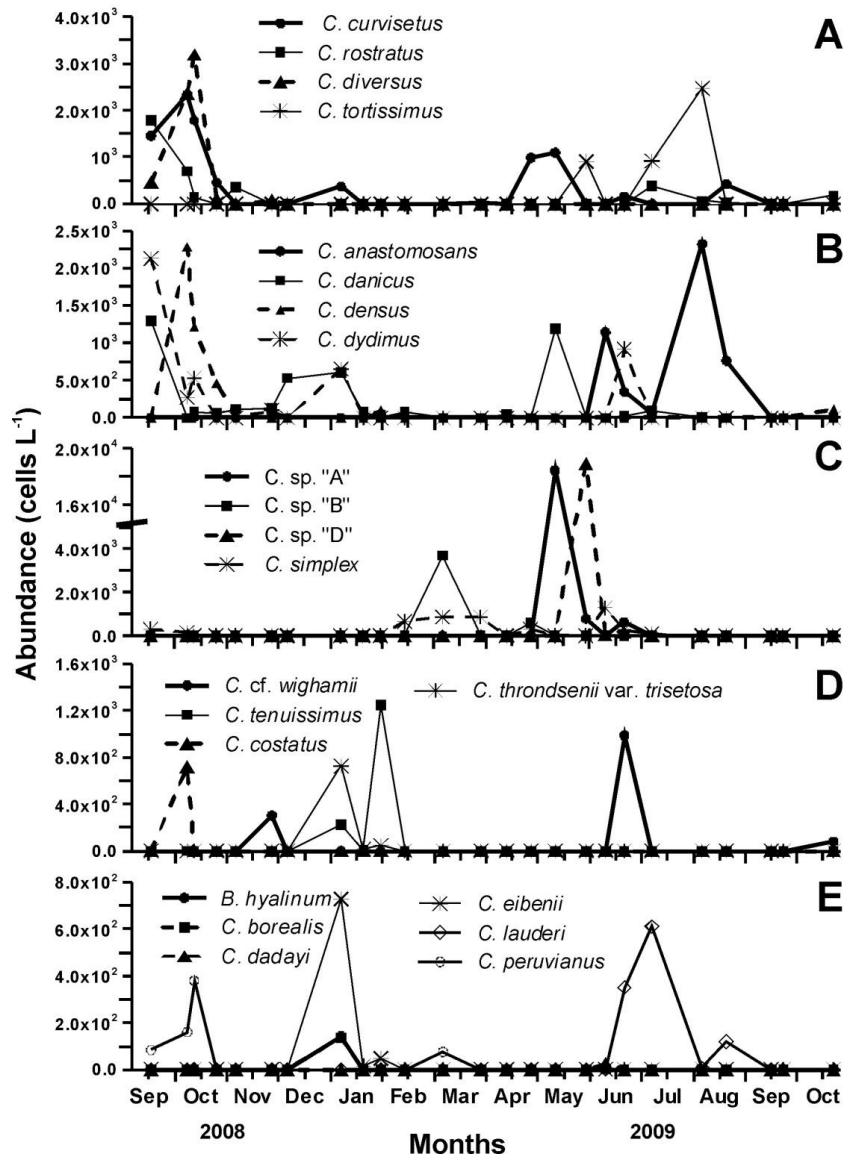
Figure 3.73. Temporal distribution of frequent and rare Chaetoceros (A-E) and Bacteriastrium (E) species abundances recorded at the station RV001 from September 2008 to October 2009.
