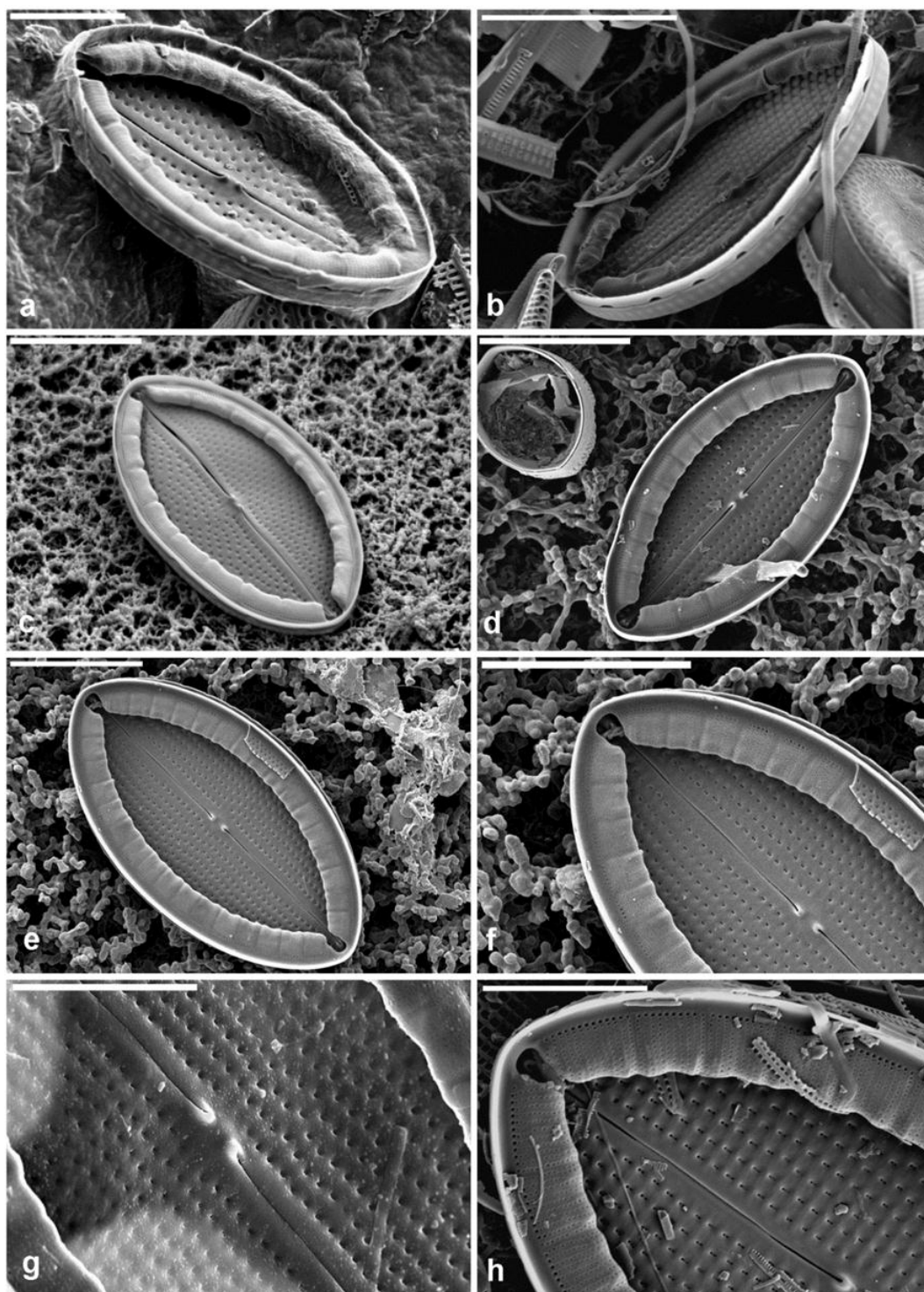
Figs a-h. Mastogloia ovulum Hustedt. Internal view. Scale bars = 10 µm (Figs b, c, d, e, f, g); 5 µm (Figs a, h).
