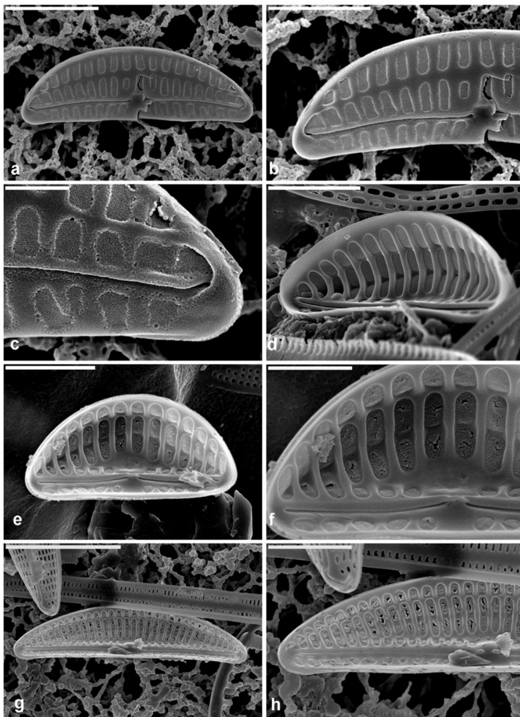
Figs a-h. SEMs of Amphora sp. Scale bars = 5 µm (Fig. g); 3 µm (Fig. a); 2 µm (Figs b, d, e, h); 1 µm (Fig. f); 500 nm (Fig. c).
