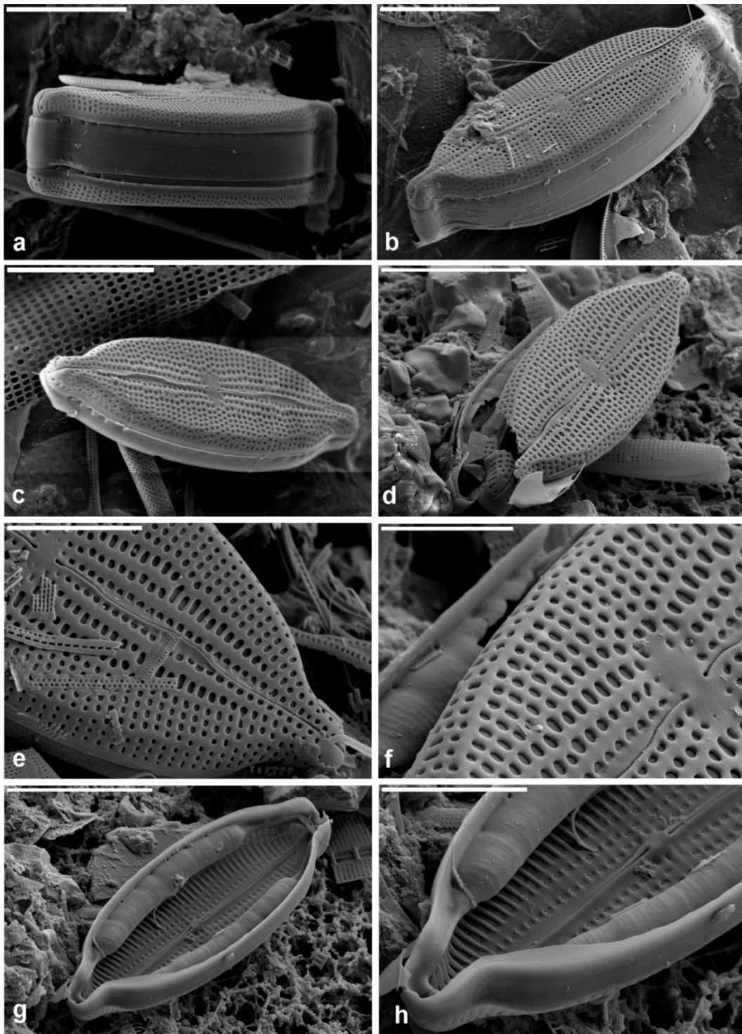
Figs a-h. Mastogloia ignorata Hustedt, Figs a-f. External valve view, Figs g-h. Internal valve view SEM. Scale bars = 10 µm (Figs a, b, c, d, g), 5 µm (Figs e, h), 3 µm (Fig. f).
