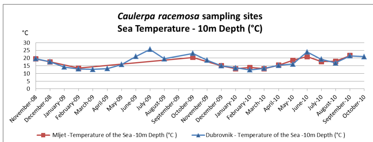
Figure 8. Temperature of the sea (°C) at the Caulerpa racemosa sampling sites from November 2008 till October 2010.
