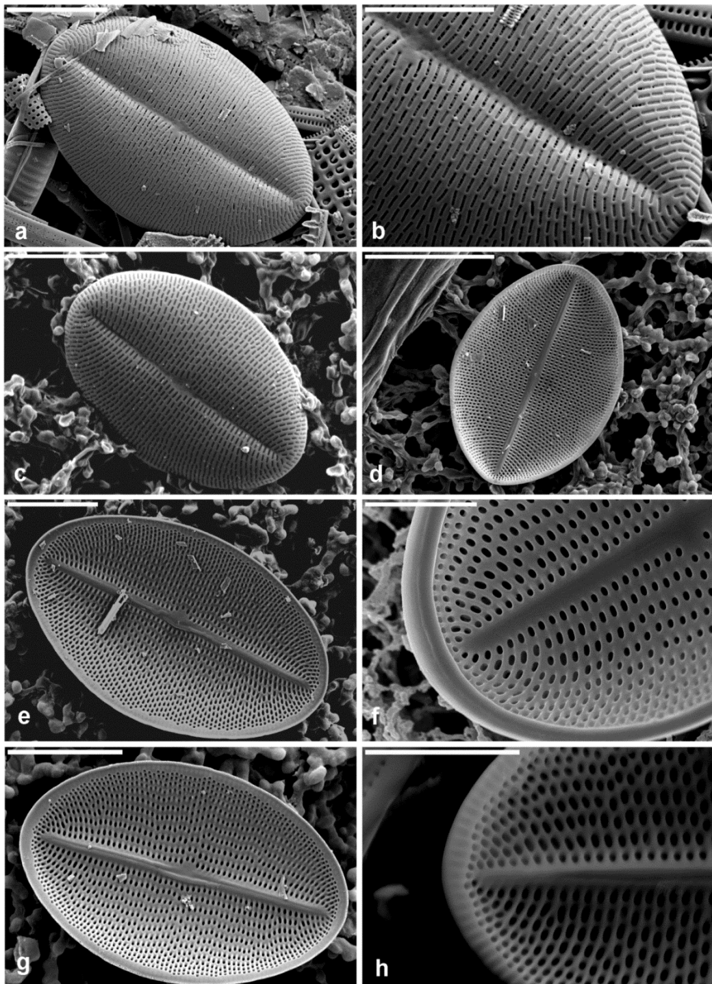
Figs a-h. Cocconeis molesta var. crucifera Greunow in Van Heurck (SEM). Figs a-c. Sternal valves, external view; Figs d-h. Sternal valves, internal view. Scale bars = 10 µm (Fig. d); 5 µm (Figs a, c, e, g); 3 µm (Figs b, h); 2 µm (Fig. f).
