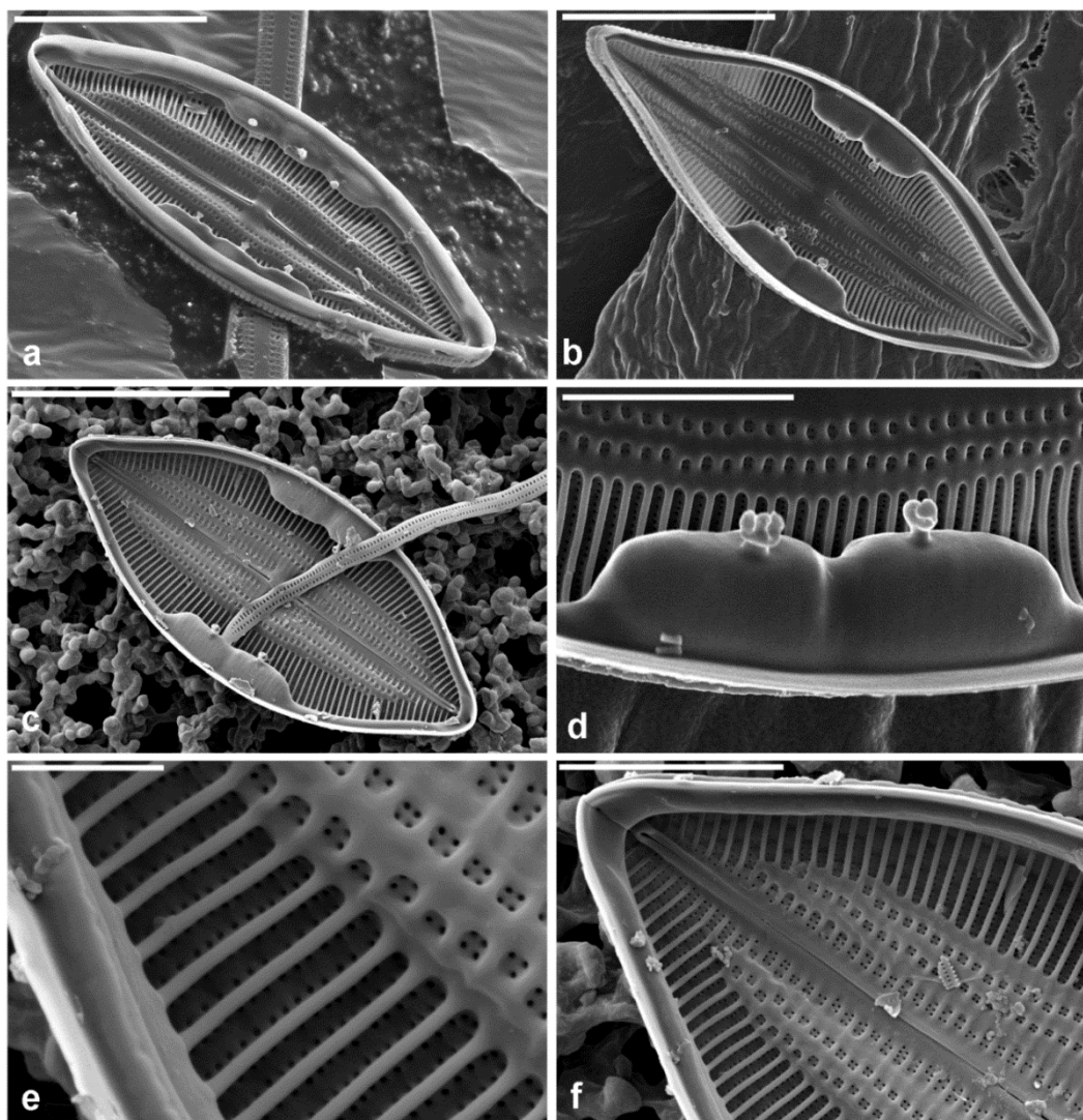
Figs a-f. Mastogloia exilis Hustedt, Internal valve view, SEM. Scale bars = 10 \mu\text{m} (Figs a, b, c); 4 \mu\text{m} (Fig. f); 3 \mu\text{m} (Fig. d); 1 \mu\text{m} (Fig. e).
