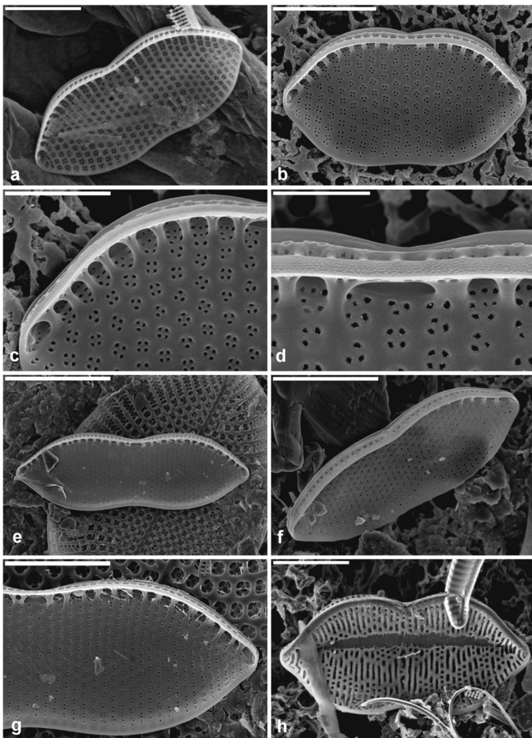
Figs a-h. SEMs of Nitzschia spp. Figs a-d. Nitzschia (SEM); Figs e-g. Nitzschia coarctata Grunow var. continua ; Fig. h. Nitzschia cf. coarctata Grunow. Scale bars = 10 µm (Fig. e); 5 µm (Figs a, f, g, h); 4 µm (Fig. b); 2 µm (Fig. c); 1 µm (Fig. d).
