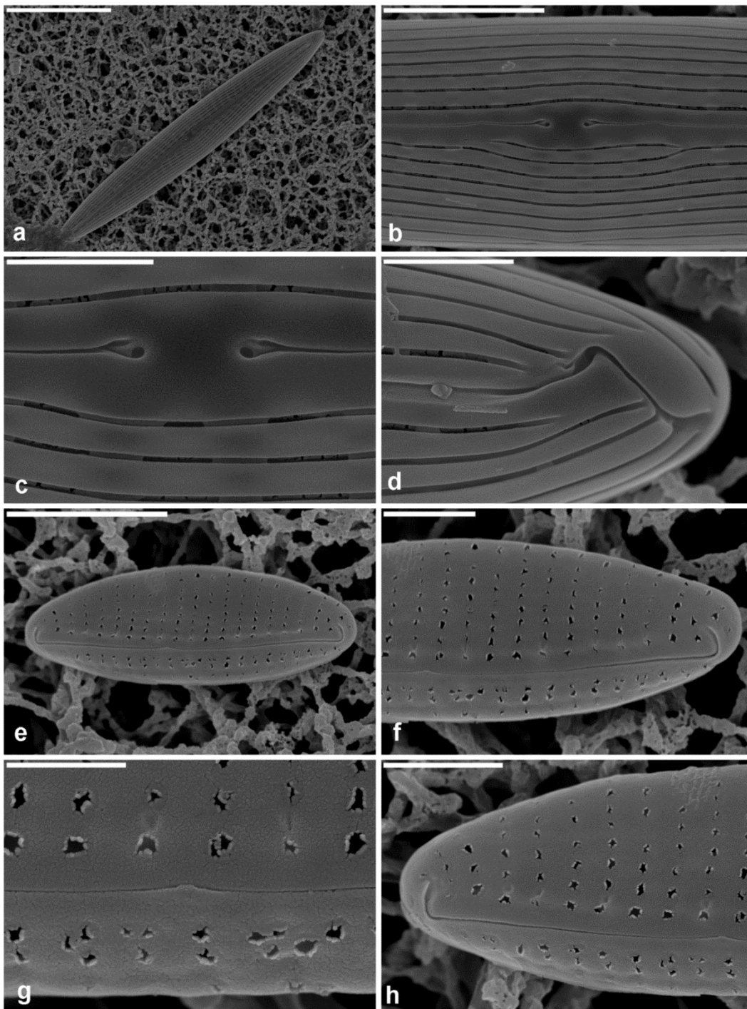
Figs a-d. Navicula subagnita Proshkina-Lavrenko (SEM). Figs e-h. Nitzschia sp. (SEM). Scale bars = 10 µm (Fig. a); 3 µm (Figs b, e); 1 µm (Figs c, d, f, h); 500 nm (Fig. g).
