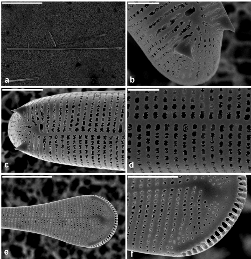
Figs a-f. Licmophora sp.(SEM). Scale bars = 100 \mu\text{m} (Fig. a); 5 \mu\text{m} (Fig. e); 2 \mu\text{m} (Figs c, f); 1 \mu\text{m} (Figs b, d).
