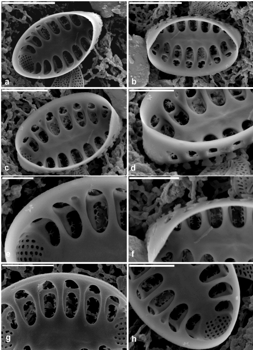
Figs a-h. Plagiogrammatea gen. et sp. nov. Scale bars = 4 \mu\text{m} (Figs a, b); 3 \mu\text{m} (Fig. c); 2 \mu\text{m} (Figs d, f, g, h); 1 \mu\text{m} (Fig. e).
