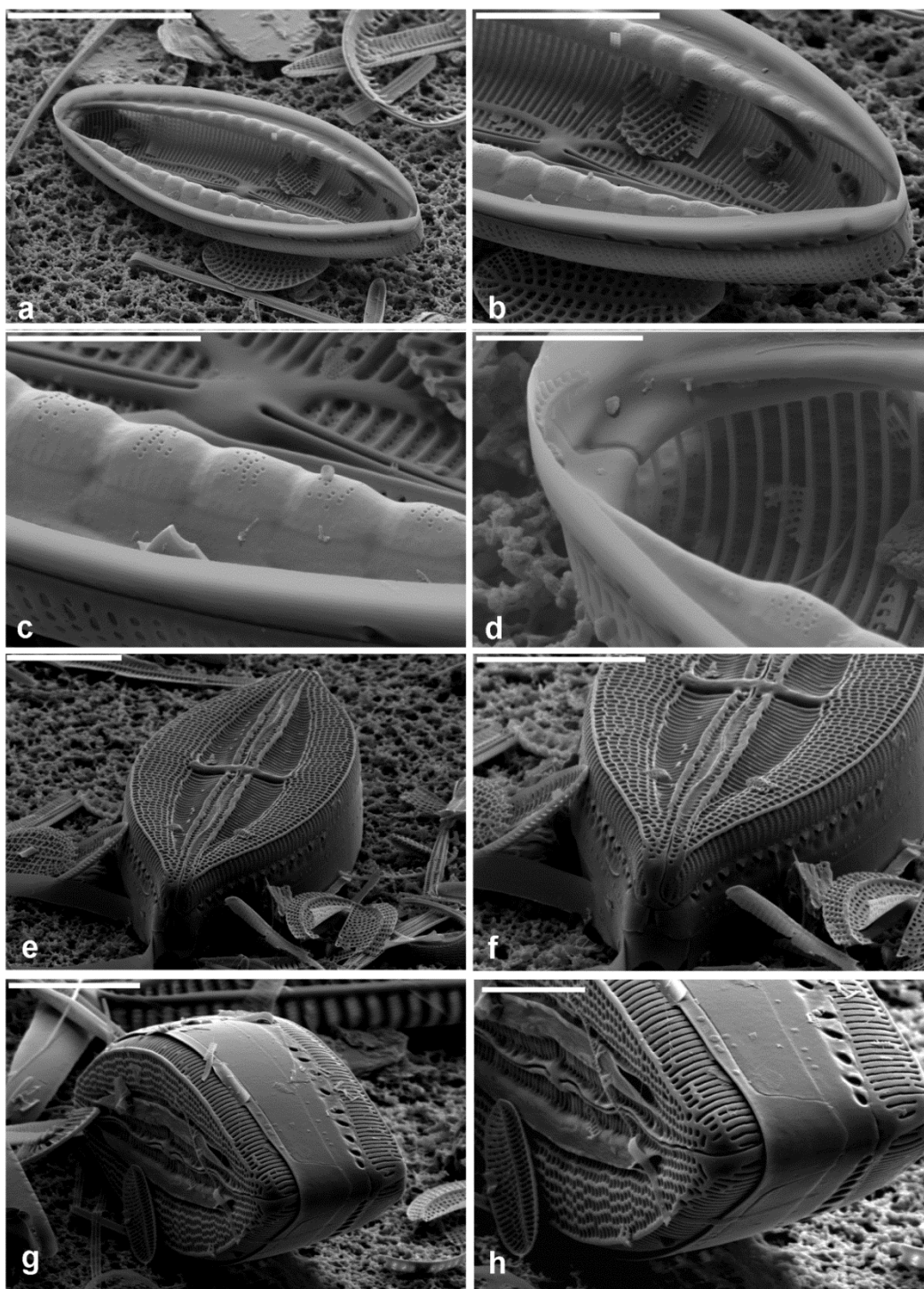
Figs a-d. SEMs of Mastogloia spp. Figs a-d. Internal view. Figs. e-h. External view. Scale bars = 20 \mu m (Fig. a); 10 \mu m (Figs b, e, f, g); 5 \mu m (Fig. h); 4 \mu m (Fig. c); 3 \mu m (Fig. d).
