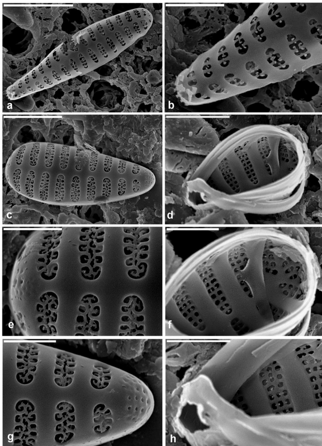
Figs a, b. Pseudostaurosira sp. (SEM). Figs c-h. Opephora sp. nov. (SEM). Scale bars = 3 µm (Figs a, c); 2 µm (Fig. d); 1 µm (Figs b, e, f, g, h).
