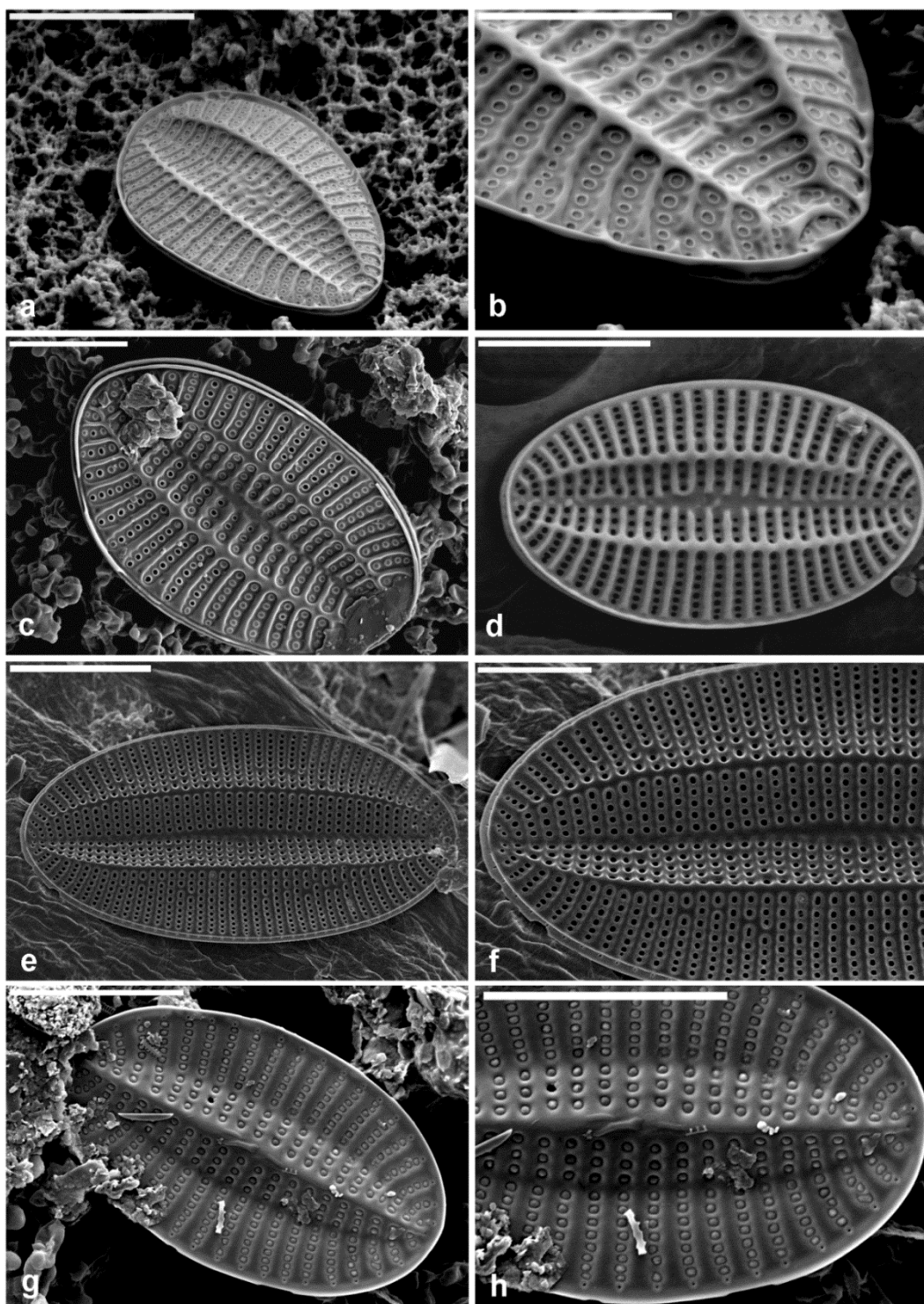
Figs a-f. Cocconeis peltoides Hustedt (SEM). Scale bars = 10 μm (Figs a, e); 5 μm (Figs c, d, g, f, h); 4 μm (Fig. b).
