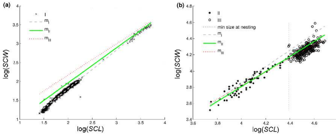
Figure 2.3: Predictions of \log(SCW) by regression equations ' m_I ', ' m_{II} ', and ' m_{III} '. Regression equations are specific for life stage subsets 'I', 'II', and 'III' (respectively). Panel (a): subset 'I', panel (b): subsets 'II' and 'III'. Parameters for the equations are provided in Table 2.5.
