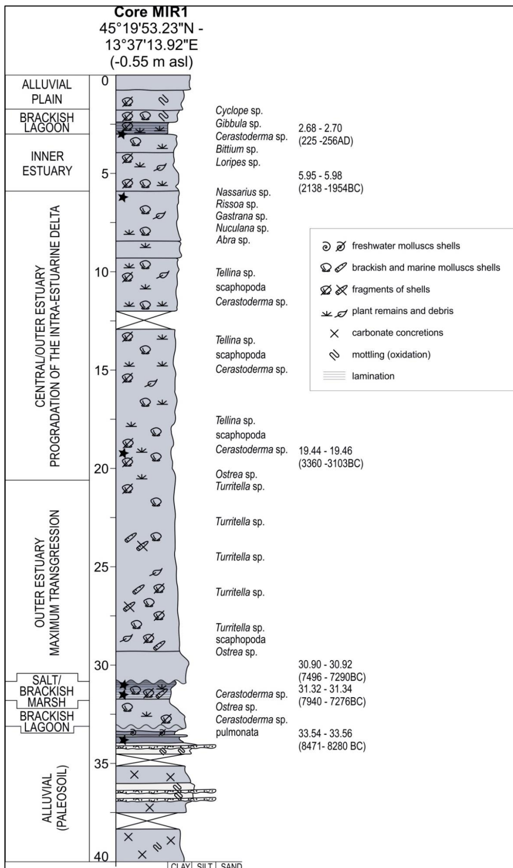
Figure 6.6. Stratigraphic log and interpretations of environment in the core MIR1
