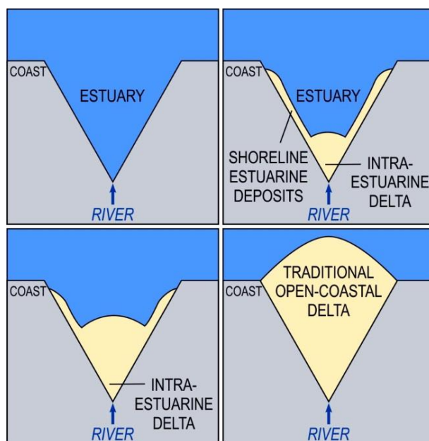
Figure 2.5. Idealized figure showing the evolution from relatively narrow V-shaped open estuary, with minimal or no sediment fill, then development of intra-estuarine delta and stronger sedimentation inside estuary, to a coastal delta where sedimentary accretion has prograded into the marine environment. Intra-estuarine deltas are present and more clearly evident in estuaries where sediments have not fully occluded them (modified after Kennish, 2016).
