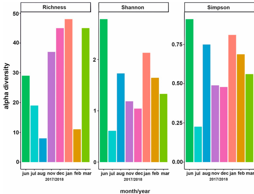
Figure 4. Alpha diversity of the richness, Shannon, and Simpson indices of the phytoplankton community inferred from the morphological and molecular approach during the investigated period ((a) = morphological approach, (b) = molecular approach).
