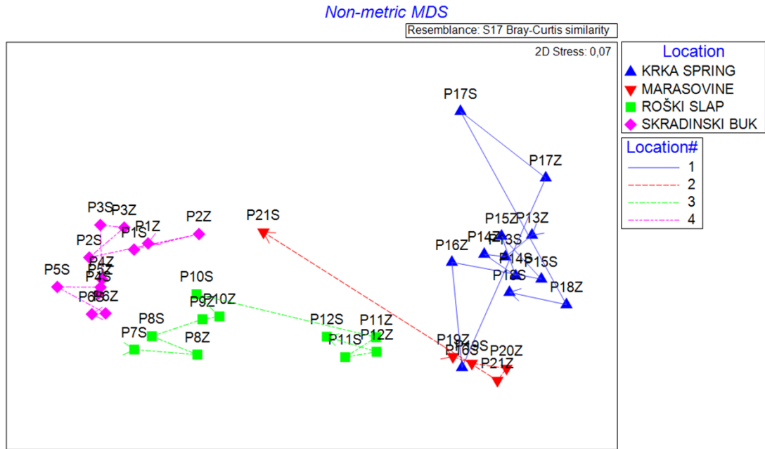
Fig. 5 Position of sampling locations in the non-metric multidimensional scaling analysis (NMDS) based on Bray-Curtis similarity index for all protist groups with categorical factor applied as the drawn trajectories, specifying all groups in the same order by the selected factors: order of sampling locations – river section parts (1-4) and location names (line type and colour represent different locations). Letters in samples name denote “Z” as light- and “S” as dark- exposed side from sampled tufa/stone
