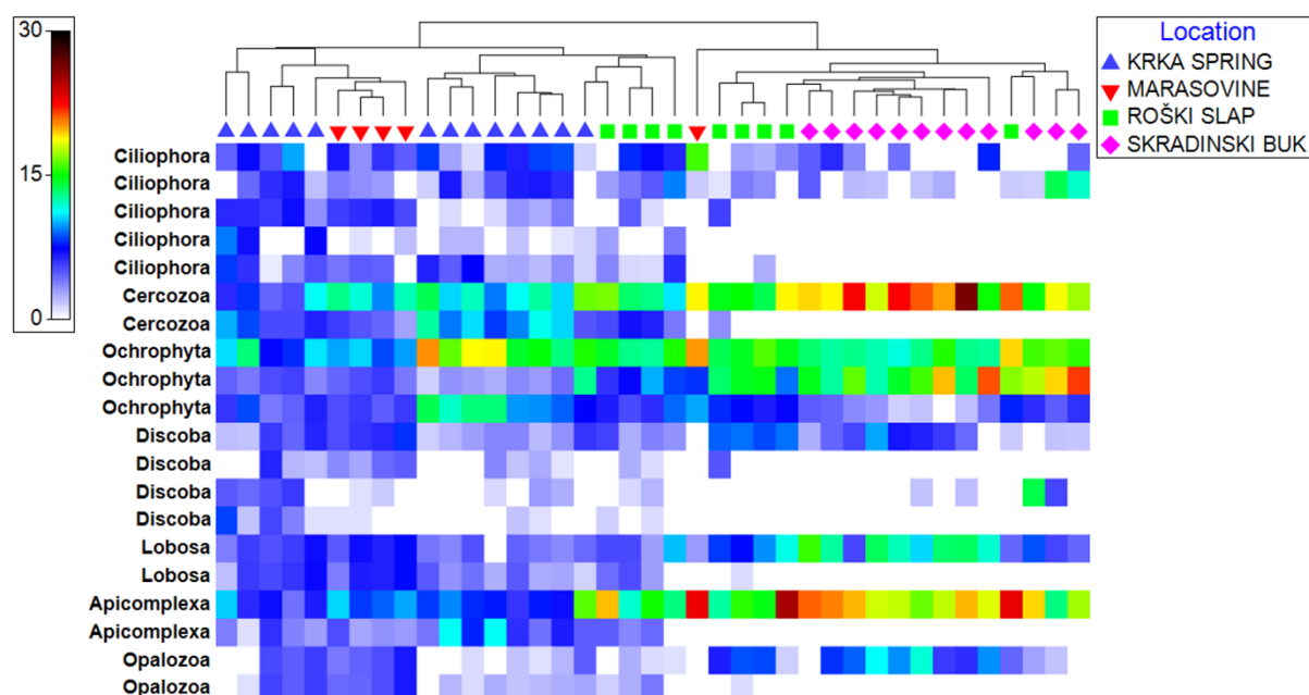
Fig. 3 Shade plot showing relationships among clusters of samples and major protist groups which contributed for at least 10% of the protists OTUs abundances
