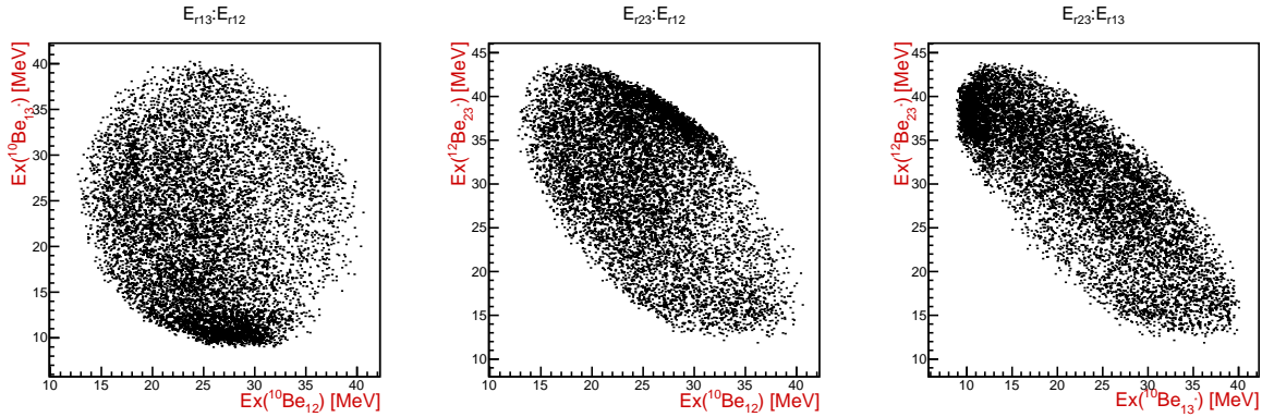
Figure 4.9: Excitation energy spectra for the {}^{10}\text{Be}_{12} , {}^{10}\text{Be}_{13}^* and {}^{12}\text{Be}_{23}^* , from the {}^7\text{Li}({}^9\text{Li}, {}^4\text{He}({}^6\text{He})_d\text{T}=3){}^6\text{He}^* reaction. The {}^4\text{He}+{}^6\text{He} pair was detected in d\text{T}=3 combination, while undetected {}^6\text{He}^* is in the 1.8 MeV ( 2^+ ) excited state.
