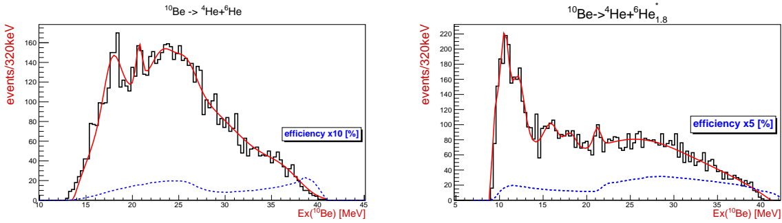
Figure 4.10: Excitation energy spectra for the {}^{10}\text{Be}_{12} (left) and {}^{10}\text{Be}_{13}^* (right), from the {}^7\text{Li}({}^9\text{Li}, {}^4\text{He}({}^6\text{He})_{d\text{T}=3}){}^6\text{He}^* reaction. Blue dashed line represents the detection efficiency curve, while the red line represents the results of the fit, with the states listed in Tables 4.5 and 4.6 respectively.
