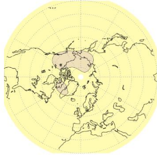
Appendix Figure C3 Signal variance (sig var) of geopotential heights at 200 hPa [ \text{m}^2 ] in the 57 non-ENSO years in January (left), February (middle), and March (right) in the ICTP AGCM experiments: Ctrl, TroAtl, TroInd, TroPac, Tropics, and Clim, respectively. The non-ENSO years were selected from 156 years (1855-2010) according to the strength of the Niño3.4 index in the JFM season.
