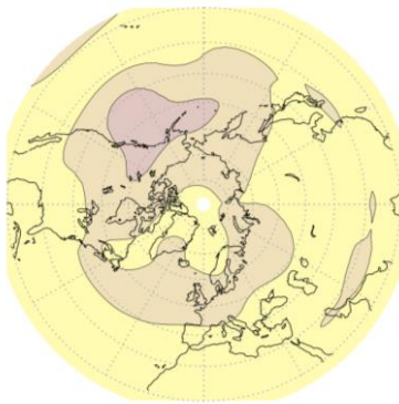
Appendix Figure D3 Signal variance (sig var) of geopotential heights at 200 hPa (GH200) [ m^2 ] in the 57 non-ENSO years in January (left), February (middle), and March (right) in the Ctrl and 2xCO2 ICTP AGCM experiments. The non-ENSO years were selected from the 156 years (1855-2010) according to the strength of the Niño3.4 index in the JFM season.
