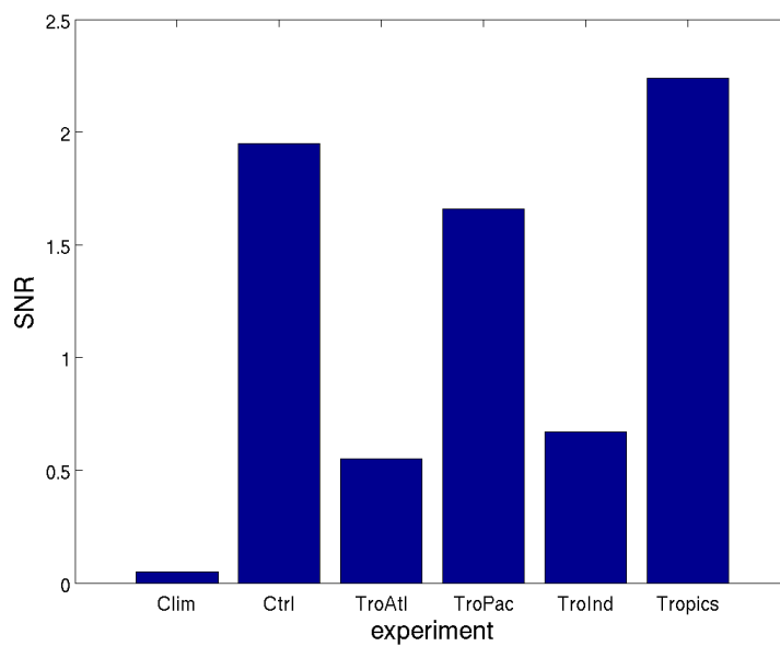
Figure 4.6 First optimal pattern (EOF1) of JFM geopotential heights at 200 hPa (GH200) [m] in the period 1855-2010 in the ICTP AGCM experiments:(a) Clim, (b) Ctrl, (c) TroAtl, (d) TroInd, (e) TroPac, and (f) Tropics. Signal-to-noise ratio (SNR) of the EOF1 mode (4.6g). All SNR values are considered statistically significant according to the F-test for the ratio of variances at the 95% confidence level.
