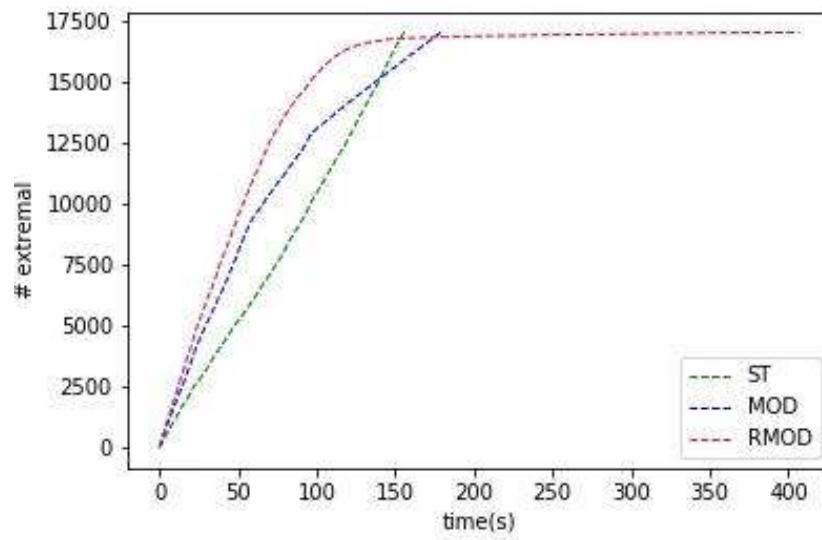
Figure 2.2: Comparison of the standard method (ST), the modified algorithm with lexicographic traversal (MOD), and the modified algorithm with random choice of B (RMOD), on residue code [16, 6, 4]
