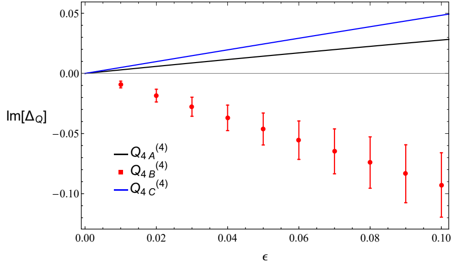
Figure 19: The imaginary part of the scaling dimension for the U(4) \times U(4) operators with CSD \bar{Q} = 4 , carrying the charges \mathcal{Q}_{4A}^{(4)} (black line), \mathcal{Q}_{4B}^{(4)} (red dots) and \mathcal{Q}_{4C}^{(4)} (blue lines) at the fixed point values as a function of \epsilon . The error bars encode the numerical error in evaluating \Delta_0 for \mathcal{Q}_{4B}^{(4)} .
