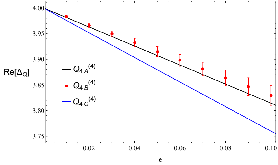
Figure 18: The results for the real part of scaling dimension for the U(4) \times U(4) operators with CSD \bar{Q} = 4 , carrying the charges \mathcal{Q}_{4A}^{(4)} (black line), \mathcal{Q}_{4B}^{(4)} (red dots) and \mathcal{Q}_{4C}^{(4)} (blue lines) as a function of \epsilon . The error bars encode the numerical error in evaluating \Delta_0 for \mathcal{Q}_{4B}^{(4)} .
