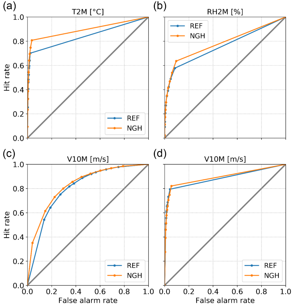
Fig. 37. ROC curves averaged over all forecast ranges of REF (blue) and NGH (orange) for (a) T2M (threshold: > 32\text{ }^{\circ}\text{C} ), (b) RH2M (threshold: > 90\% ), (c) W10M (threshold: > 2\text{ ms}^{-1} ) and (d) W10M (threshold: > 8\text{ ms}^{-1} ) for the verification period.
