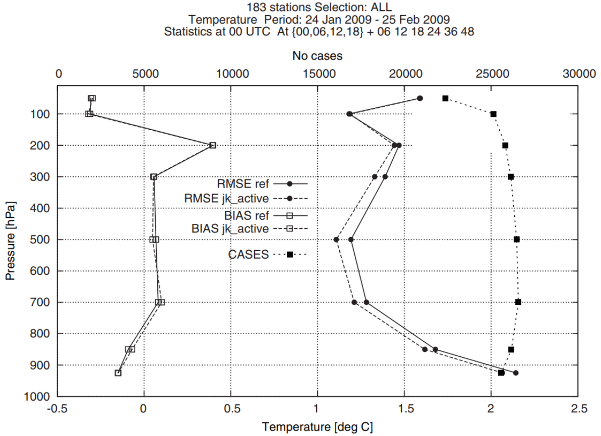
Fig. 2. Figure 12. from Dahlgren and Gustafsson (2012). Verification of temperature forecasts compared with observations from radiosondes. To the right is the root mean square error and to the left the mean error (bias) averaged over all forecast ranges, valid at 00 UTC. Full line: reference experiment (i.e., without Jk ). Dotted line: reference with Jk blending. The number of observations used in the statistics is also shown using the upper x-axis.
