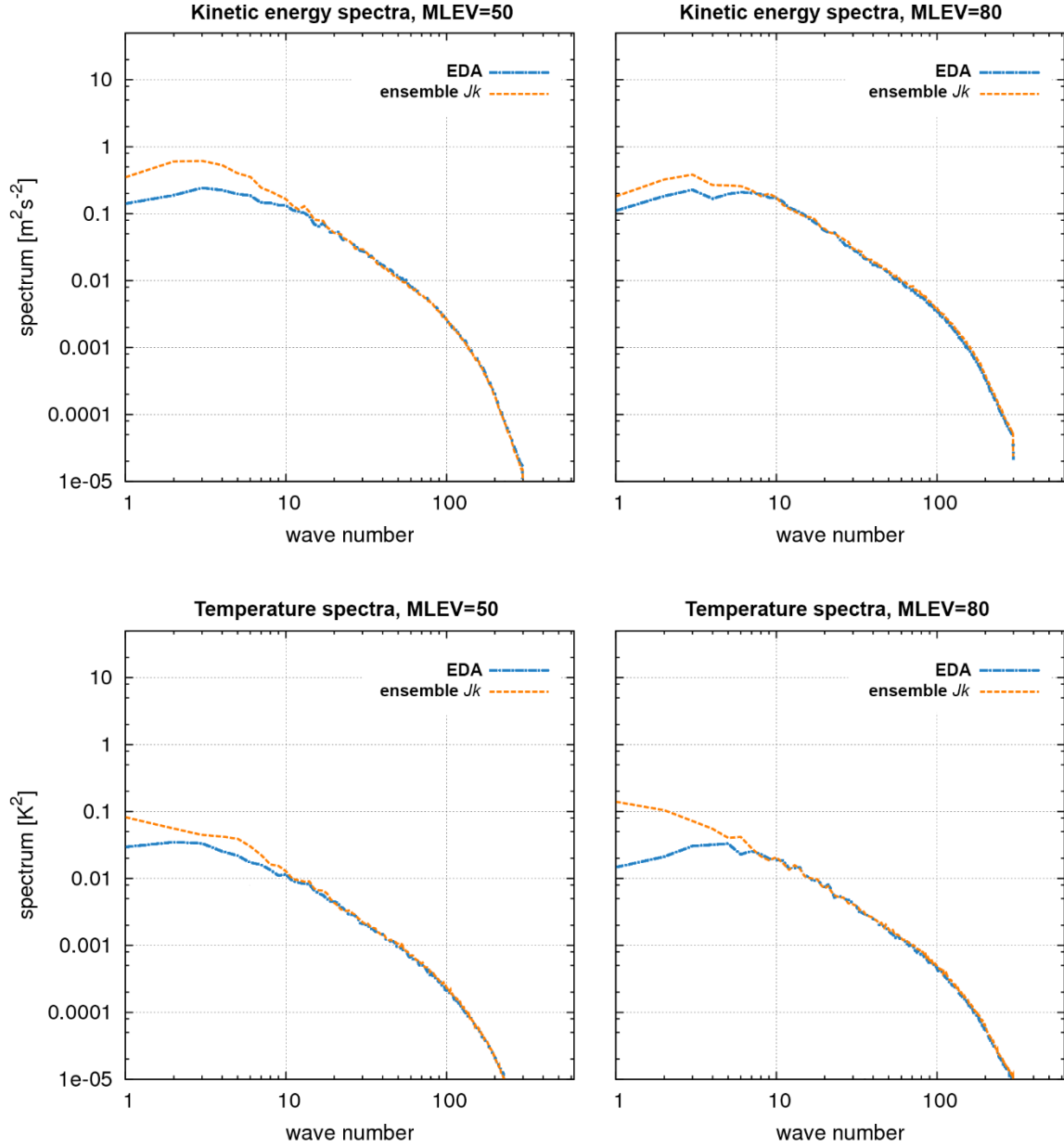
Fig. 7. Kinetic energy (upper row) and temperature (lower row) spectra at model levels 50 (left column) and model level 80 (right column) averaged over the period of 7 days, two times per day. EDA perturbations (blue) and ensemble Jk perturbations (orange). Denoted wave numbers 10 and 100 correspond to wavelengths of about 150 km and 15 km, respectively.
