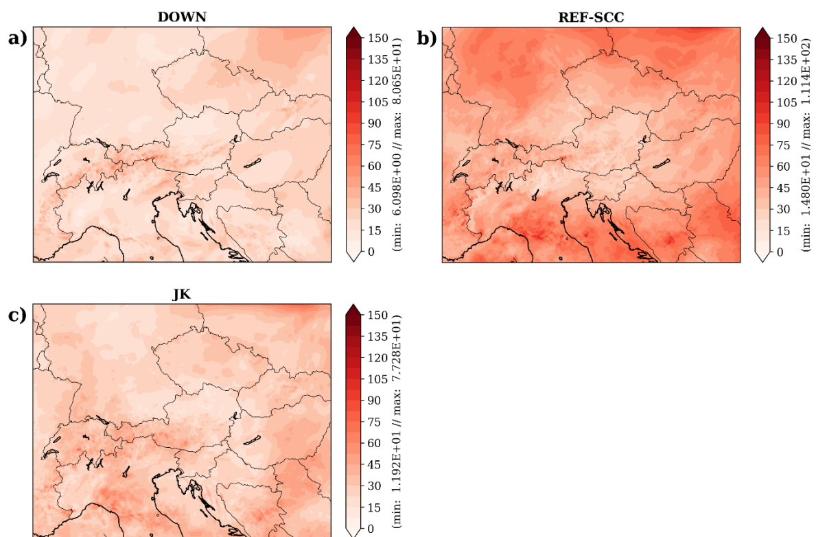
Fig. 31. As Fig. 29. but for 15 July at 0100 UTC.
