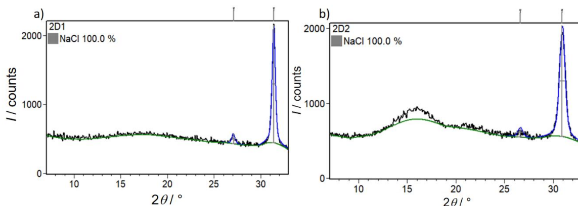
Figure 42. Rietveld refinement on samples 2D1 and 2D2 obtained by the reaction involving \text{NaBH}_4 , \text{ZnCl}_2 and \text{NaIm} in ratio: a) 1:1:1 and b) 1:1:3. Experimental diffraction data are shown in black, while calculated patterns are given in blue. Position of diffraction lines corresponding to sodium chloride are given by grey vertical marks.
