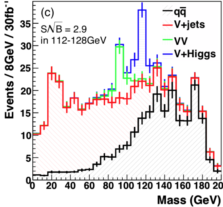
Figure 2.7: Expected signal and background distributions for a 115 GeV SM Higgs in boosted topology ( W(l\nu)H(bb) channel) according to calculation in BDRS paper.
