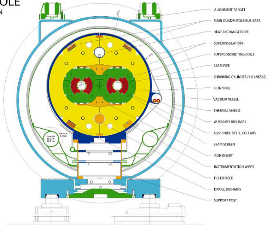
Figure 3.3: Schematic cross section of a LHC dipole magnet.
