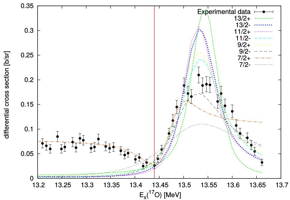
Figure 3.32: Different spin and parity combinations for the peak at 13.6 MeV using a single resonance without a background. The best shape and height of the peak is obtained for \frac{11}{2}^- . See text for details.
