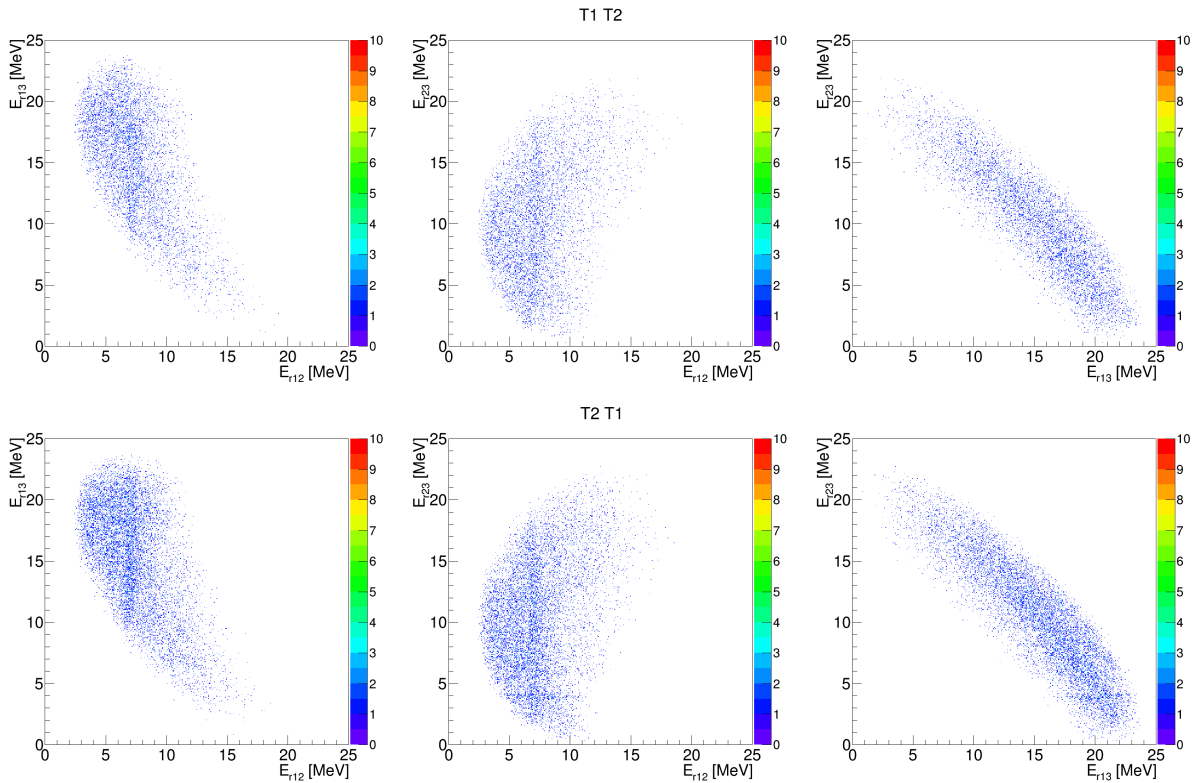
Figure 4.72: Relative-energy plots for the {}^9\text{Be}({}^{13}\text{C}, {}^8\text{Be}_{\text{gs}} {}^4\text{He}){}^{10}\text{Be}_{\text{gs}} reaction. Different detector combinations are displayed one per row. {}^8\text{Be}_{\text{gs}} , {}^4\text{He} and {}^{10}\text{Be} are designated by numbers 1, 2 and 3, respectively.
