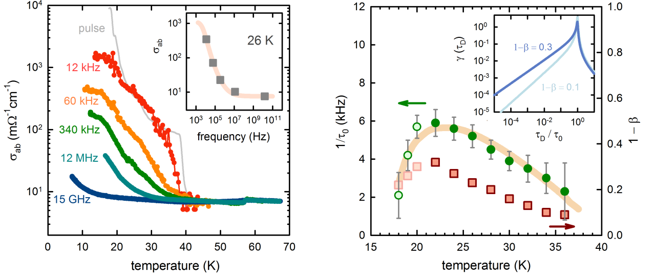
Figure 3.17: Frequency-dependent conductivity of LBCO-1/8.
