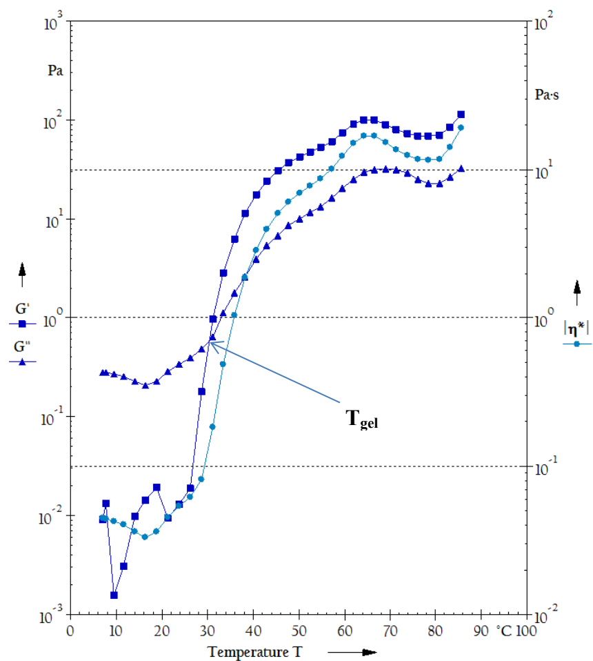
Figure 20: Typical temperature sweep profile of temperature responsive in situ forming gel ( G' - squares, G'' - triangles and \eta^* - circles). T_{\text{gel}} is marked with an arrow at intersection of G' and G'' curves.
