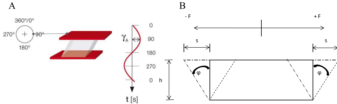
Figure 9. Oscillatory rheological test: A) two plates model to illustrate oscillatory shear tests, picture reprinted from (104); B) oscillatory tests: shear force \pm F , deflection path \pm s and deflection angle \pm \phi in the shear gap h , picture reprinted with permission from (100).
