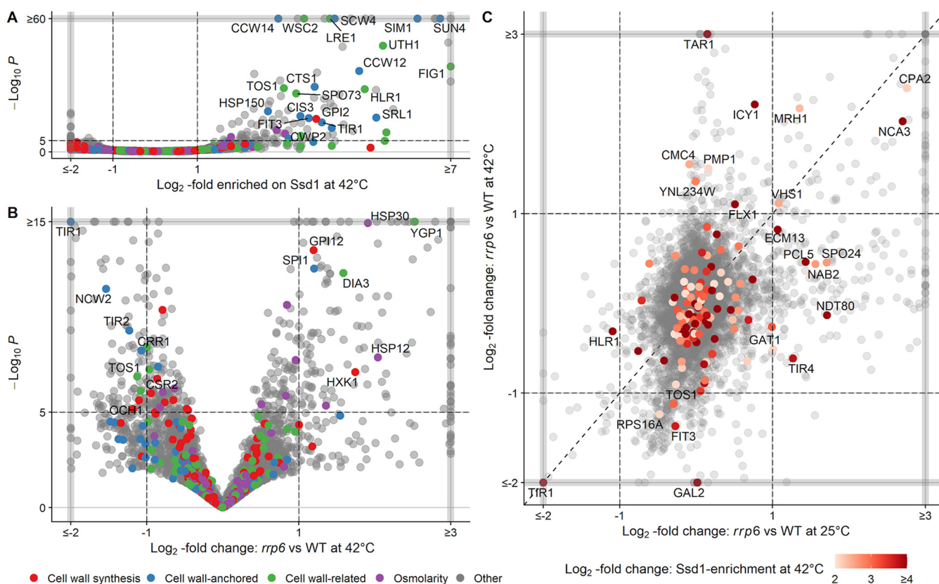
FIG 4 Volcano plots (A) showing which mRNAs are enriched for Ssd1 binding after heat stress (42°C for 16 min) (24) and (B) comparing transcriptomes of rrp6Δ versus wild-type (WT) yeast after heat stress (42°C for 10 min) (23). Different colors highlight four groups of cell-wall-associated proteins (see supplemental material). Only mRNAs belonging to these four groups of genes and more than 2-fold enriched/upregulated or depleted/downregulated ( |\log_2| fold change of \geq 1 , -\log_{10} P \geq 5 ) are highlighted. Genes within gray lines are more up- or downregulated than shown but were placed within the lines to save space. (C) Comparison of rrp6Δ versus wild-type yeast transcriptomes at 25°C (x axis) (23) and 42°C (y axis, 10 min) (23), with mRNAs highlighted in the shades of red if they are enriched for Ssd1 binding more than 4-fold ( \log_2 fold change of \geq 2 ) during heat shock (42°C for 16 min) (24) and labeled only if they are up- or downregulated by more than 2-fold ( |\log_2| fold change of \geq 1 ).
