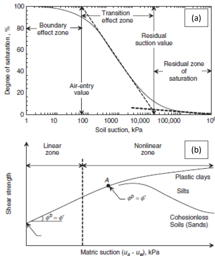
Figure 57: Relationship of SWRC to shear strength envelope for different types of soil: a) desaturation zones along the SWRC, and b) variation in shear strength envelopes for different soils in different desaturation zones (Fredlund et al. 2012).
