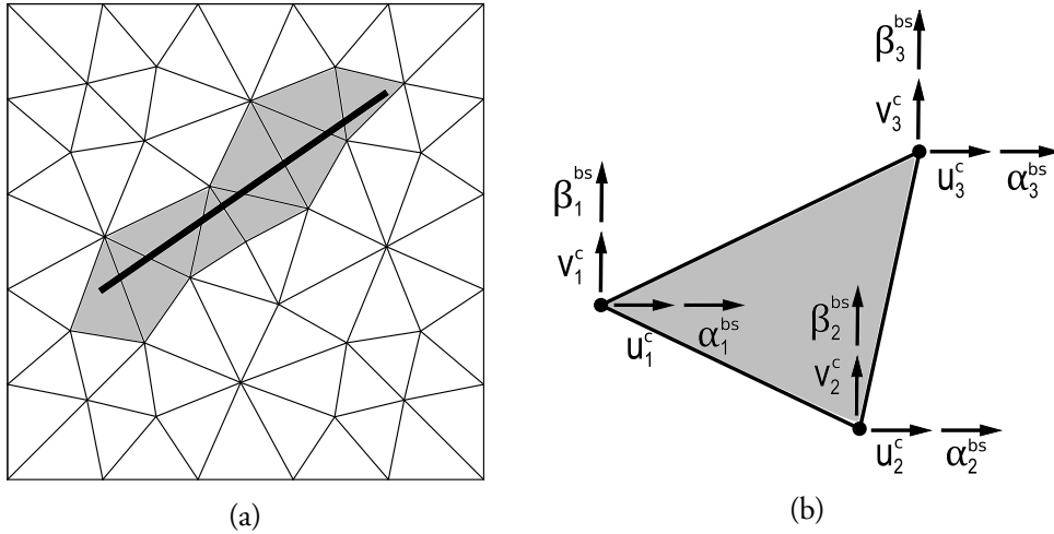
Figure 3.1: Non-conforming mesh: (a) a randomly oriented fiber in the domain; (b) degrees of freedom of a fully enriched element.
