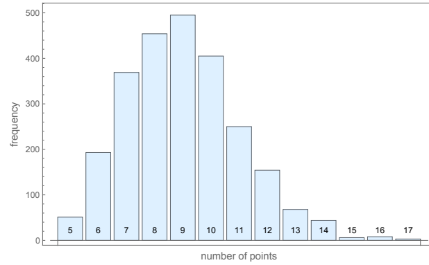
Figure 4.10: Frequency of appearance of numbers from table shown in Figure 4.9b.
