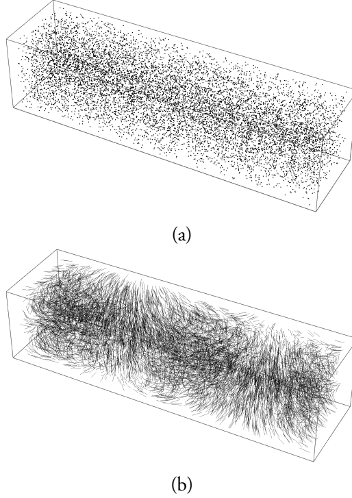
Figure 4.16: Distribution of fibers in a concrete specimen of dimensions 40x10x10 cm: (a) fiber midpoints; (b) whole fibers.
