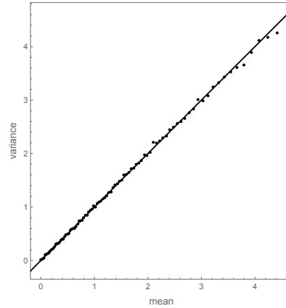
Figure 4.13: Plot of variance vs. mean in logarithmic scale for different zone sizes.
