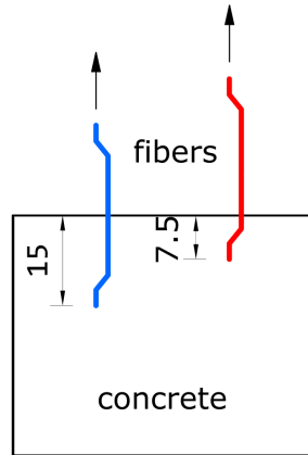
Figure 2.10: Different embedded lengths for the fiber: l^{\text{fe}} = 7.5 mm (one quarter of the fiber length), and l^{\text{fe}} = 15 mm (one half of the fiber length).
