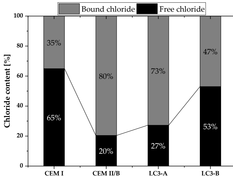
Figure 3.10 Bound and free chloride content at the depth of 10 mm from exposed surface towards salt solution
