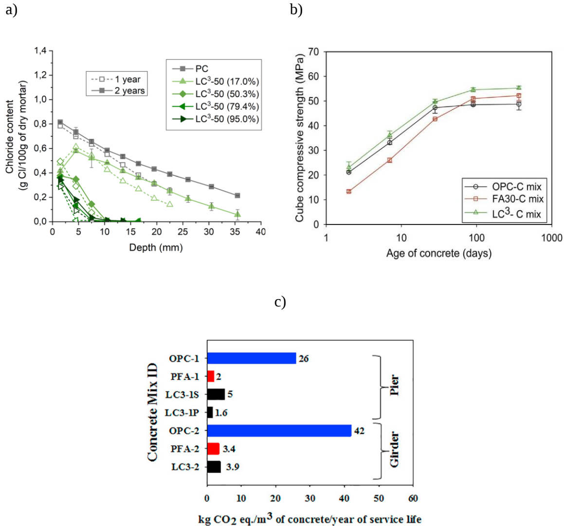
Figure 1.6 a) Chloride penetration of LC3 system with various kaolinite content [31] , b) Evolution compressive strength of LC3 compared to Portland and Fly ash systems [29] , and c) Service life of LC3 system [30]
