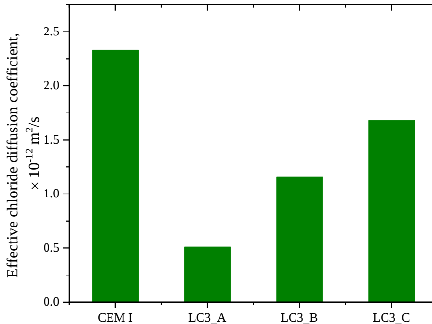
Figure 4.8 Effective chloride diffusion coefficient, D_{\text{eff}} , measured from chloride flow rate from mini migration test.
