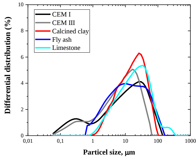
Figure 2.2 Particle-size distribution of various materials used in the study.
