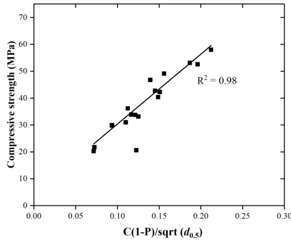
Figure 2.14 Plot of compressive strength versus pore parameters C(1-P)/\sqrt{d_{0.5}}
