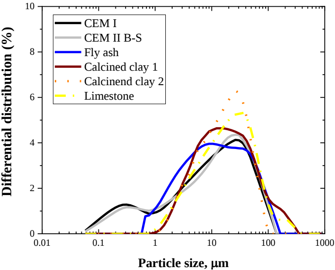
Figure 5.A.1 Particle size distribution of each binder materials
