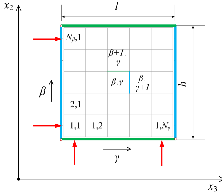
Figure 2.6: HFGMC discretization.
