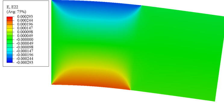
Figure 5.54: Rectangular plate - contour plot of \varepsilon_y - reference FEM solution
