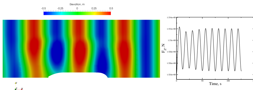
Figure 1: Free surface elevation and vertical force signal from the wave diffraction simulation.
