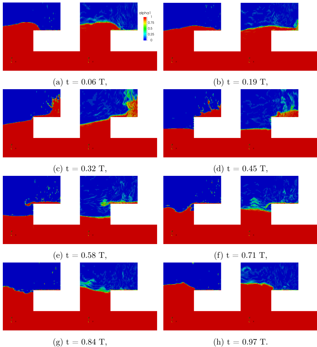
Figure 2.4: Visual comparison of the volume fraction field \alpha (denoted "alpha") in simulation where the isoAdvector (left) and the algebraic VOF method (right) are used (PAPER 5).
