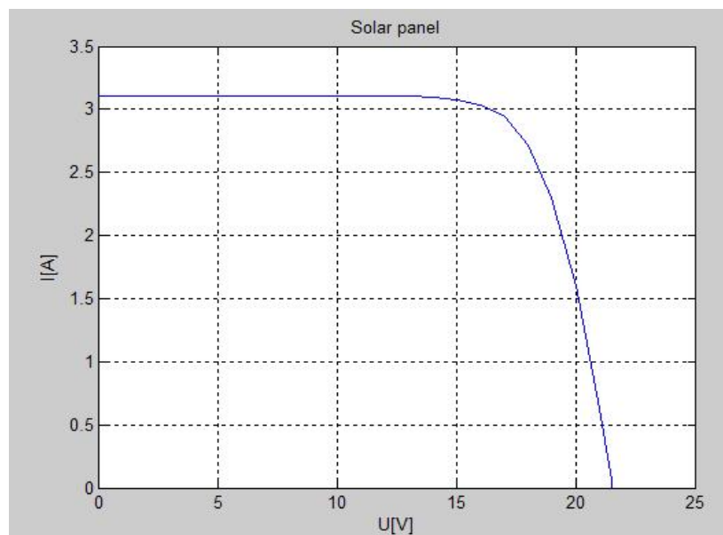
Figure 36. I-V characteristic of PV module
