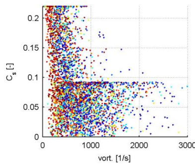
Figure 64 - Flame PSF30: scatter plot of cell values for Smagorinsky parameter C_s vs. vorticity for C_s=f(CSM) , coloured by RPV
