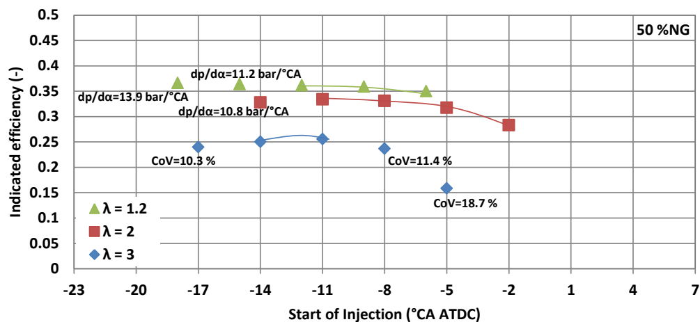
Figure 89. Influence of SOI timing on indicated efficiency for Z = 50 %NG
