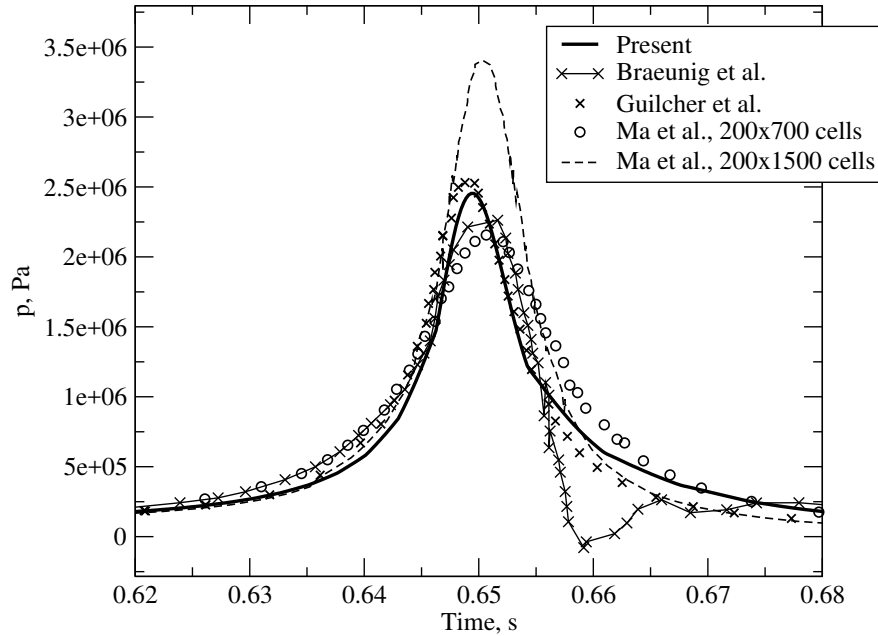
Figure 2.6: Pressure signal comparison during the impact of the falling water column. Pressure measured at the center of the bottom boundary is compared to Braeunig et al. [7], Ma et al. [8] and Guilcher et al. [9] (PAPER 6).
