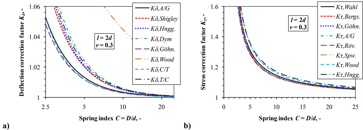
Figure 2.8. Different correction factors for \nu = 0.3 : a) deflection correction K_\delta , b) stress correction K_\tau
