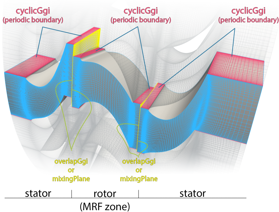
Figure 3.8: Single blade passage consisting of stator, rotor and stator with interface boundary conditions.
