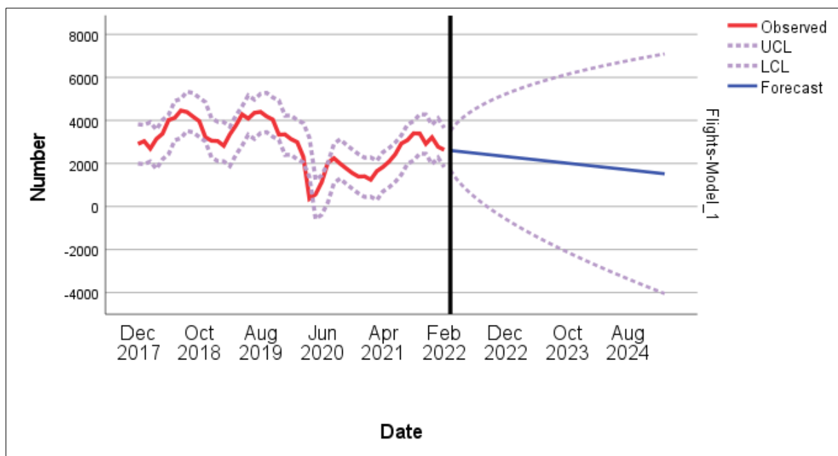
Figure 28 Example of forecasting number of flights using Holt's linear trend
