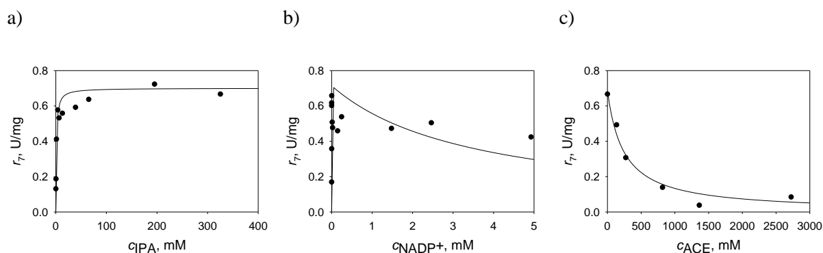
Figure 74 Kinetics of the KRED 011 -catalyzed IPA oxidation into ACE (0.1 M phosphate buffer pH 8, \gamma_{\text{KRED011}} = 0.03 mg/mL, 25 °C). The dependence of the initial reaction rate on substrates a) IPA ( c_{\text{NADP}} = 4.9 mM) and b) NADP + ( c_{\text{IPA}} = 130 mM) and c) product ACE ( c_{\text{IPA}} = 130 mM, c_{\text{NADP}} = 0.246 mM). Legend: experiment (dots), model (line).
