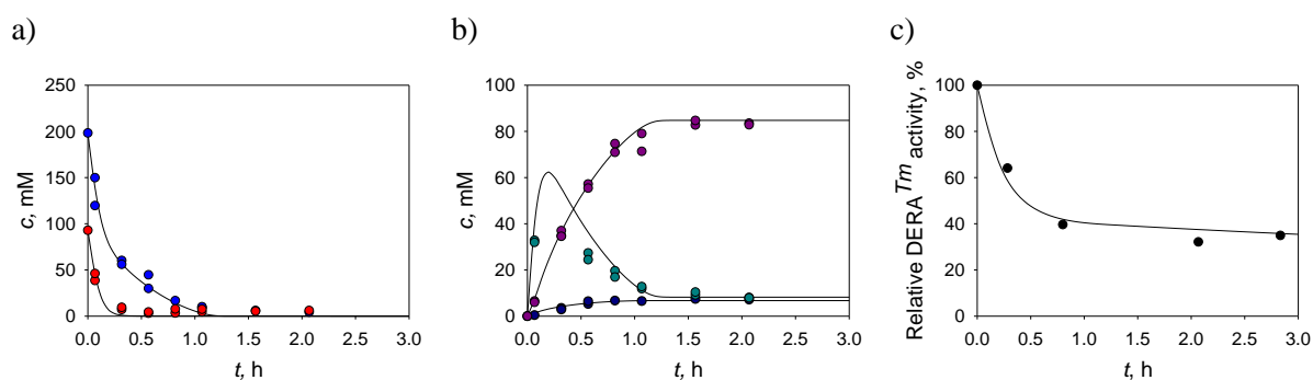
Figure 44 Experimental and simulation data of the double aldol addition of AA to CAA in a batch reactor catalyzed by DERA Tm (0.1 M TEA-HCl buffer pH 7, c_{\text{AA}} = 198 mM, c_{\text{CAA}} = 93 mM, \gamma_{\text{DERA}^{\text{Tm}}} = 10 mg/mL). Change of a) substrate concentration, b) product concentration, c) relative enzyme activity during the experiment. Legend: experiment (dots), model (line); AA (blue), CAA (red), CHB (teal), CDH (purple), CHH (dark blue).
