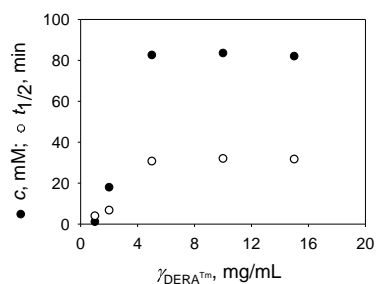
Figure 43 Enzyme half-life and concentration of CDH at different enzyme concentrations in the batch reactor ( c_{\text{AA}} = 200 mM, c_{\text{CAA}} = 100 mM, 0.1 M TEA-HCl buffer pH 7, 25 °C, \gamma_{\text{DERA}^{\text{Tm}}} = 1; 2; 5; 10; 15 mg/mL). Legend: CDH (black circles), t_{1/2} (white circles).
