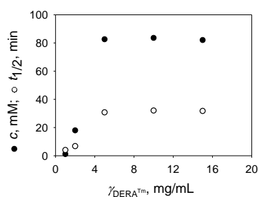
Figure 43 Enzyme half-life and concentration of CDH at different enzyme concentrations in the batch reactor ( c_{AA} = 200 mM, c_{CAA} = 100 mM, 0.1 M TEA-HCl buffer pH 7, 25 °C, \gamma_{DERA^{Tm}} = 1; 2; 5; 10; 15 mg/mL). Legend: CDH (black circles), t_{1/2} (white circles).
