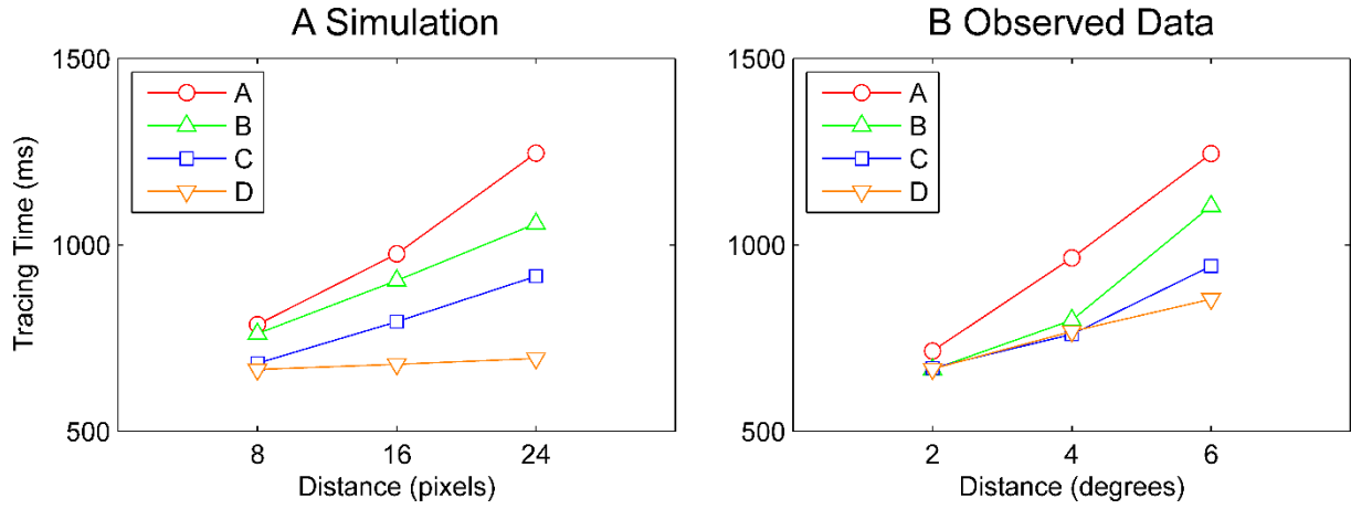
Figure 15. Comparison between the results of simulation and behavioral data. The simulated tracing times are plotted as a function of distance from the spatial cue (A). The approximately linear trend is observed with a varying slope for different levels of curvature. To compare the simulation with empirical data, in (B), we redraw mean tracing times for the same response observed in Experiment 1 of Jolicoeur et al. (1991). In their data, distance is measured in degrees of visual angle.
