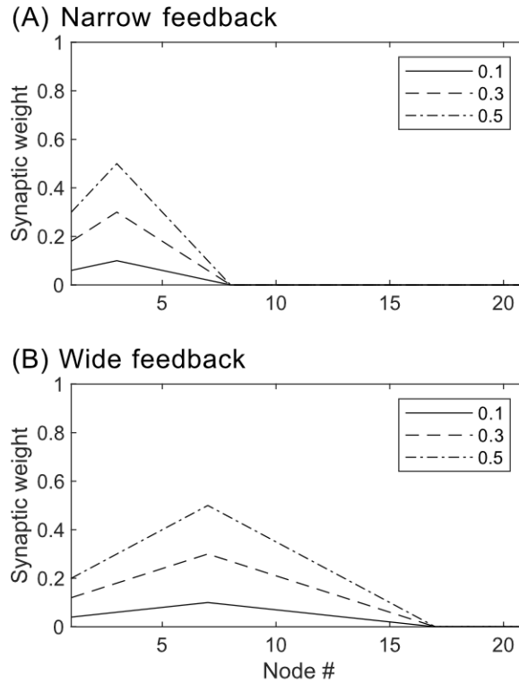
Figure 9. (A) The narrow and (B) the wide distribution of feedback signals from the inter-ART associative map to the F_2 layer were considered in simulations with three levels of the feedback gain factor.
