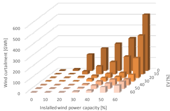
Fig. 7. Wind curtailment interdependence on wind and EV penetration EV penetration in non flexible thermal scenario and G2V charging mode
