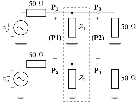
Figure 4.40: Schematic of the differential signal transmission path characterization setup used to evaluate the impact of the port-to-ground path impedance asymmetry on the common-mode rejection ratio.
