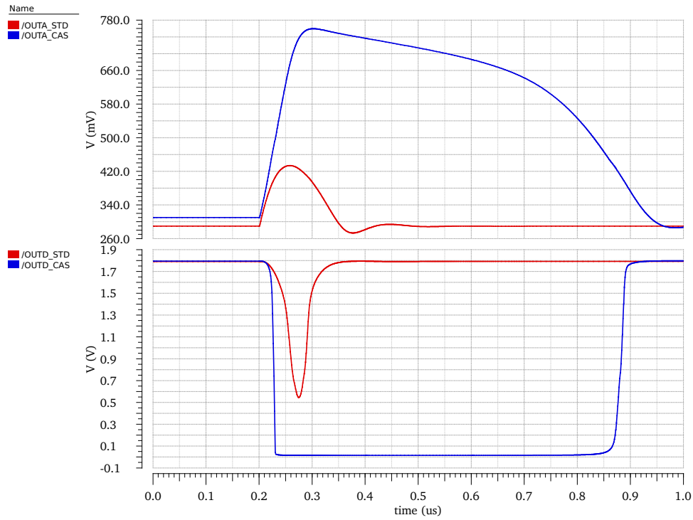
Figure 5.2: Comparison of simulated waveforms on OUT_A and OUT_D between the miniMALTA enlarged front-end and the new cascoded design with an input charge of 200\text{ e}^- . The gain of the cascoded front-end is a factor of 3 higher.
