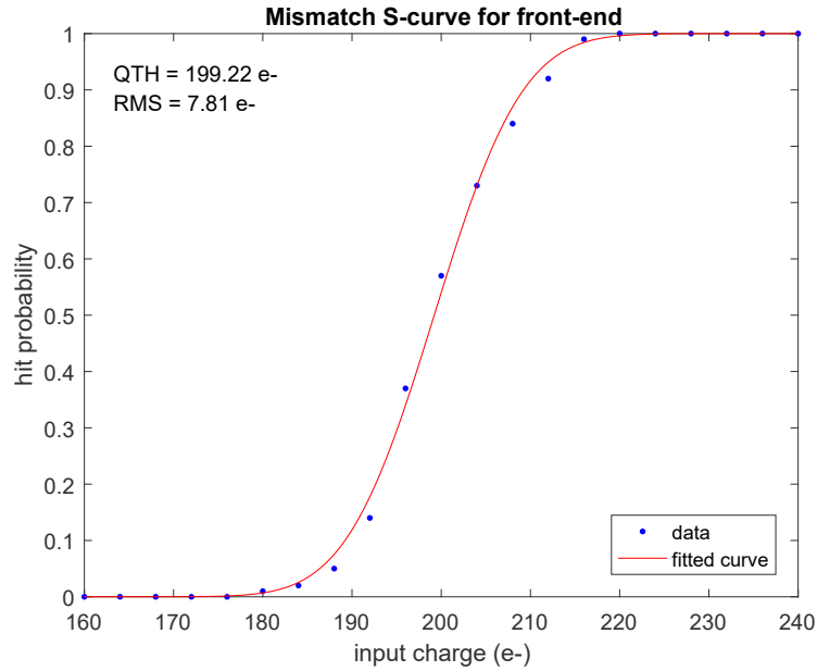
Figure 3.14: Simulated mismatch S-curve for the front-end. The RMS value of the fit yields around 8\text{ e}^- of threshold variation at a 200\text{ e}^- threshold.
