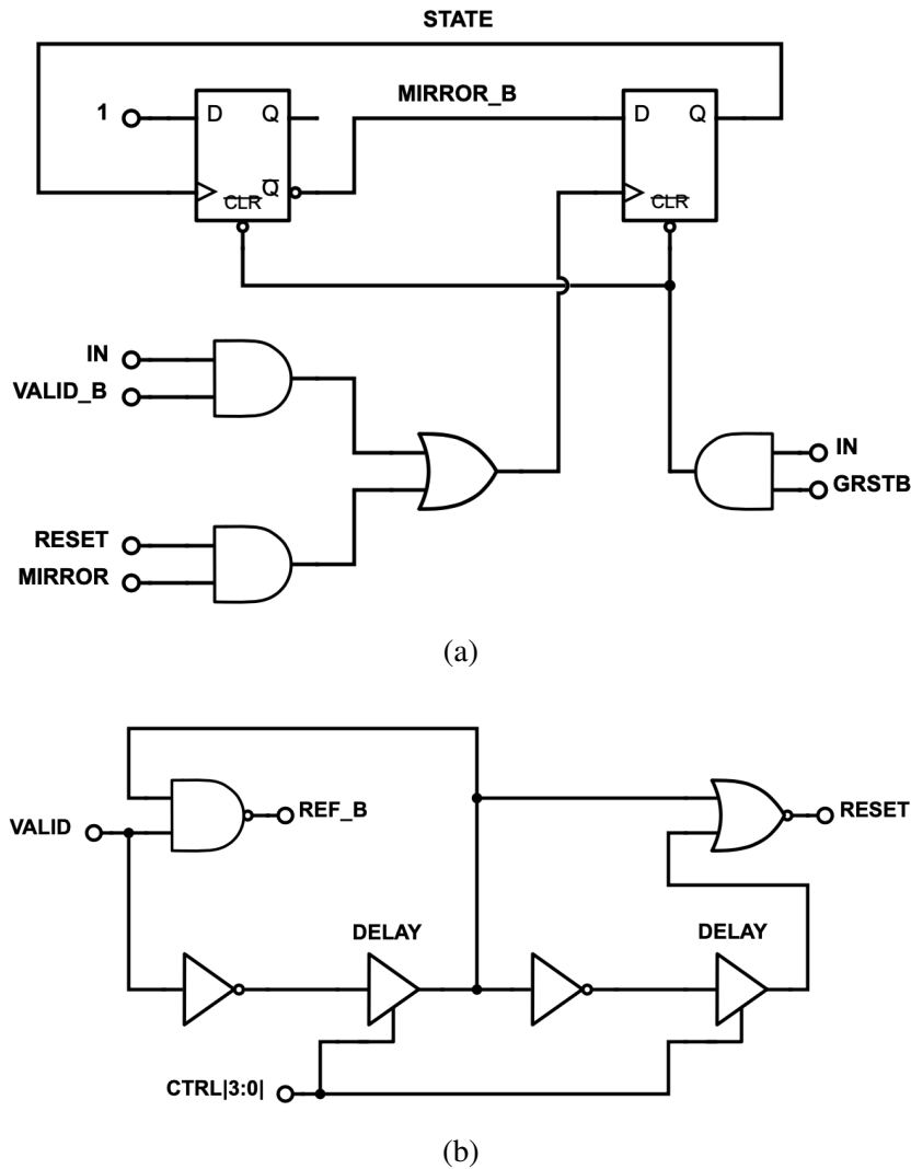
Figure 3.19: A simplified view of the in-pixel readout logic implemented in MALTA: (a) double flip-flop structure for hit arbitration (b) pulse generator circuit used to generate the reference pulse.
