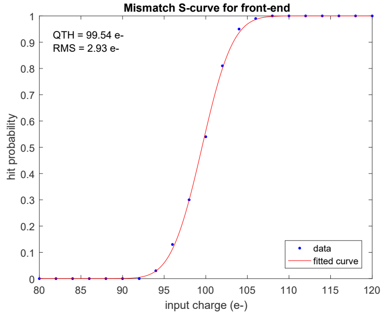
Figure 5.3: Simulated mismatch S-curve for the front-end with cascode. At a threshold setting of 100\text{ e}^- , the mismatch RMS is reduced by a factor of 2.7 compared to the front-end implemented in miniMALTA.
