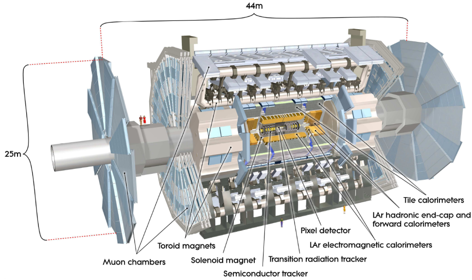
Figure 1.2: A cut-away view of the ATLAS experiment and its sub-parts (reproduced from [2]).
