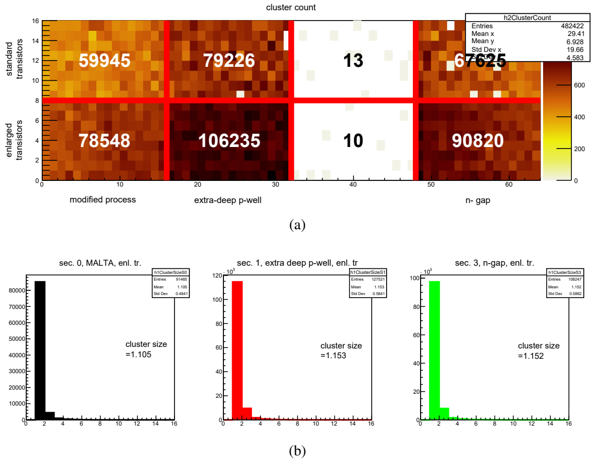
Figure 4.15: (a) Cluster occupancy and (b) cluster size distribution for different sectors with enlarged transistors in miniMALTA after 10^{15} \text{ n}_{\text{eq}}/\text{cm}^2 .
