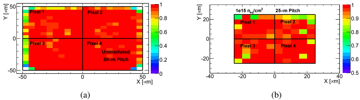
Figure 3.4: Detection efficiency across the 2 \times 2 pixel group for: (a) unirradiated 50 \times 50 \mu m 2 pixel with 3 \mu m electrode and 18.5 \mu m spacing, (b) 10^{15} neq/cm 2 irradiated 25 \times 25 \mu m 2 pixel with 3 \mu m electrode and 3 \mu m spacing.
