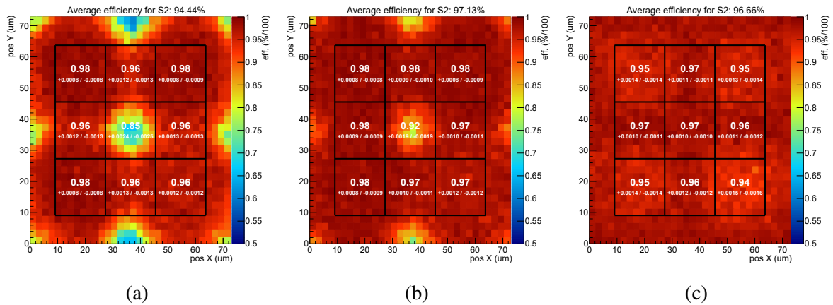
Figure 3.37: In-pixel efficiency for 2 \times 2 pixel groups at different thresholds: (a) threshold of 450\ \text{e}^- , (b) threshold of 350\ \text{e}^- , c) threshold of 250\ \text{e}^- .
