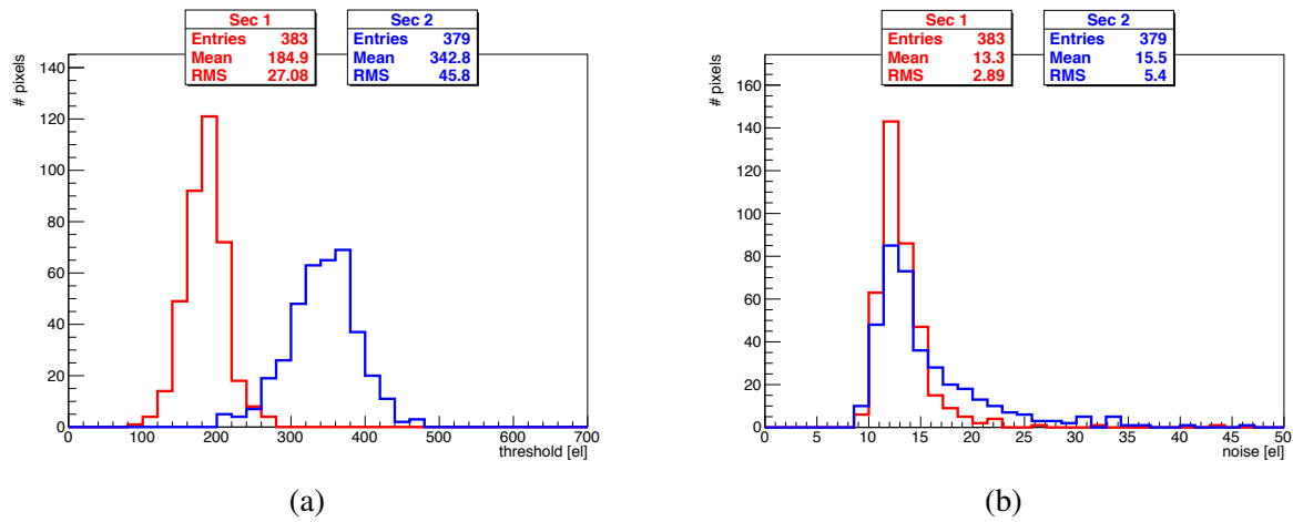
Figure 4.13: Threshold and noise distributions for the two sectors of a miniMALTA chip irradiated with neutrons to 10^{15} \text{ n}_{\text{eq}}/\text{cm}^2 .
