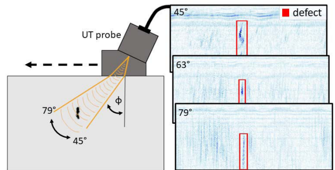
Fig. 1. Illustration of UT scanning with a phased array probe. Examples of B-scans that are obtained for various angle values are shown on the right side of the figure. Red bounding boxes mark the defect's location.
