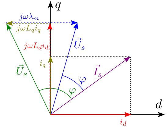
Fig. 3: Voltage phasor diagram of SyRM (green) and PMASR (blue) for a given stator current (stator resistance is neglected R_s = 0 ) [11].
