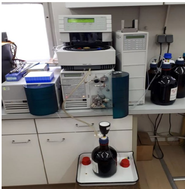
Figure 12. Varian ProStar 500 HPLC system used in quantification of extracted pyrethrins.
