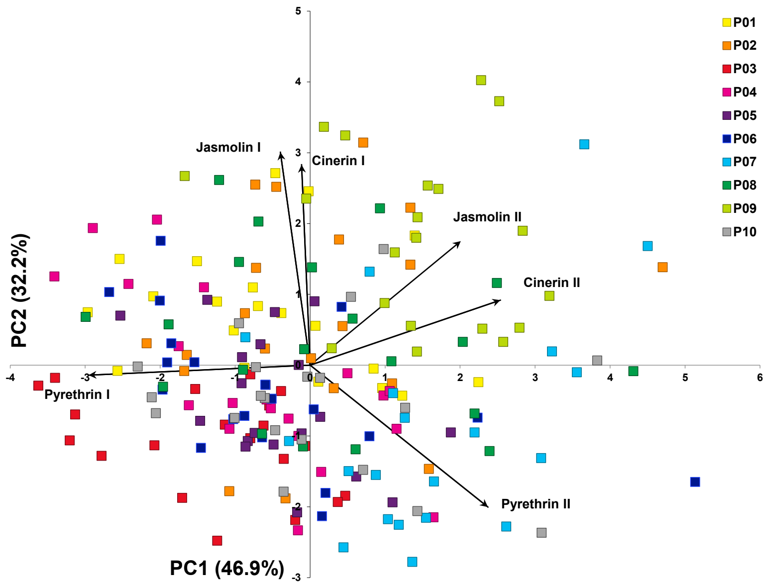
Graph 5. Biplot of Principal component analysis based on pyrethrin content.
