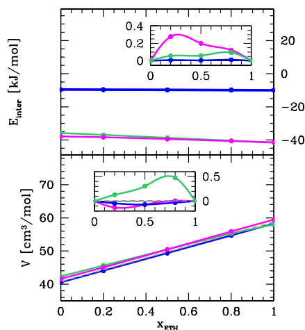
Figure 4.7.: Interpolated intermolecular energies (upper panel), molar volumes (lower panel) and corresponding excess quantities (insets) for the studied systems. Green for the OPLS model, magenta for the TraPPE model, and blue for the LJ model. The experimental data for the volumes and excess volumes [164] are equally shown in dashed grey lines.
